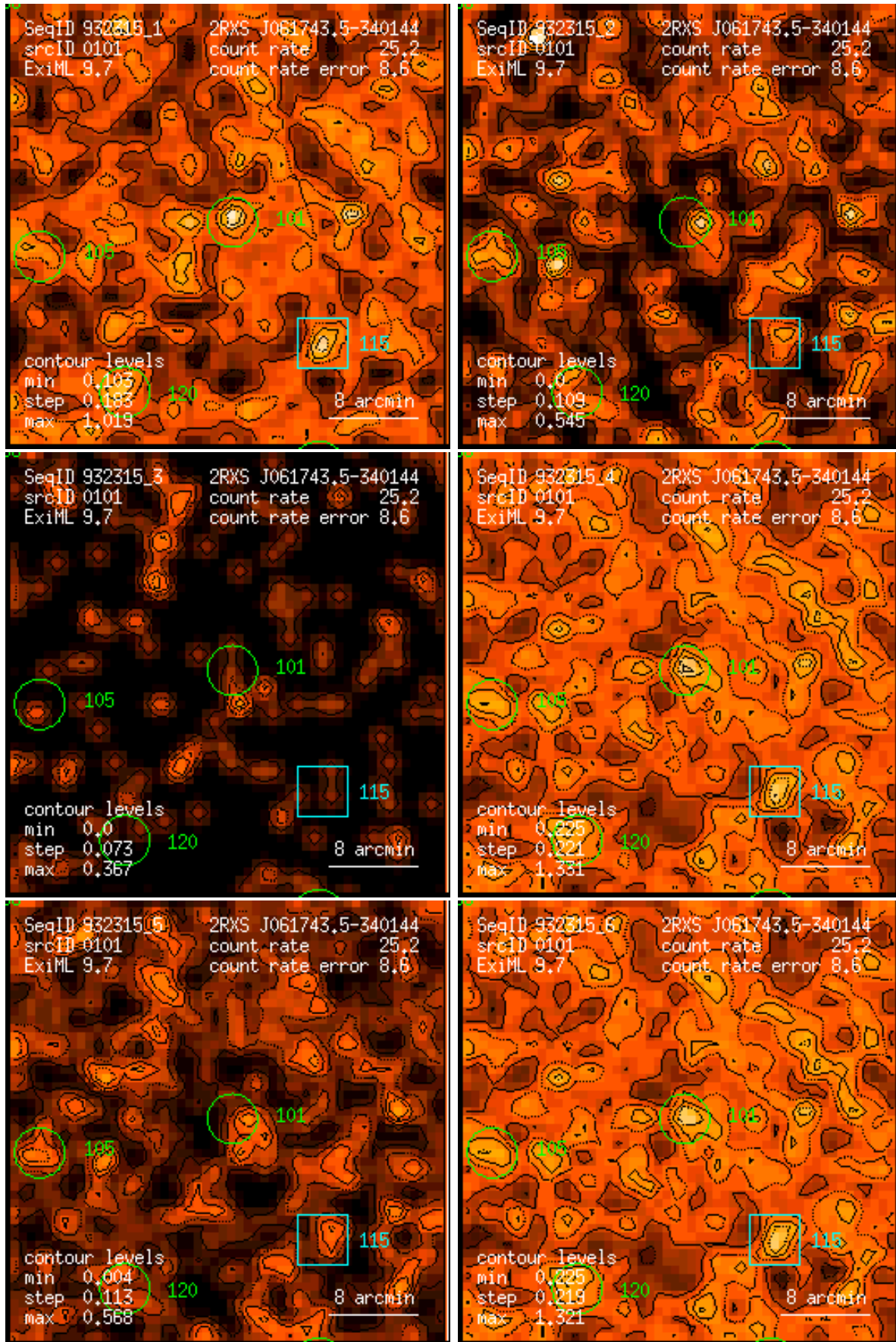
Figure 101: RASS 932315: detection 0101: band rate images, Gaussian filter: (1) PSPC channels 11 – 41, (2) 52 – 90, (3) 91 – 201, (4) 11 – 235, (5) 52 – 201, (6) 11 – 201. Broad band rates in counts/ks. Band rate contour levels in counts/ks/arcmin 2 .
