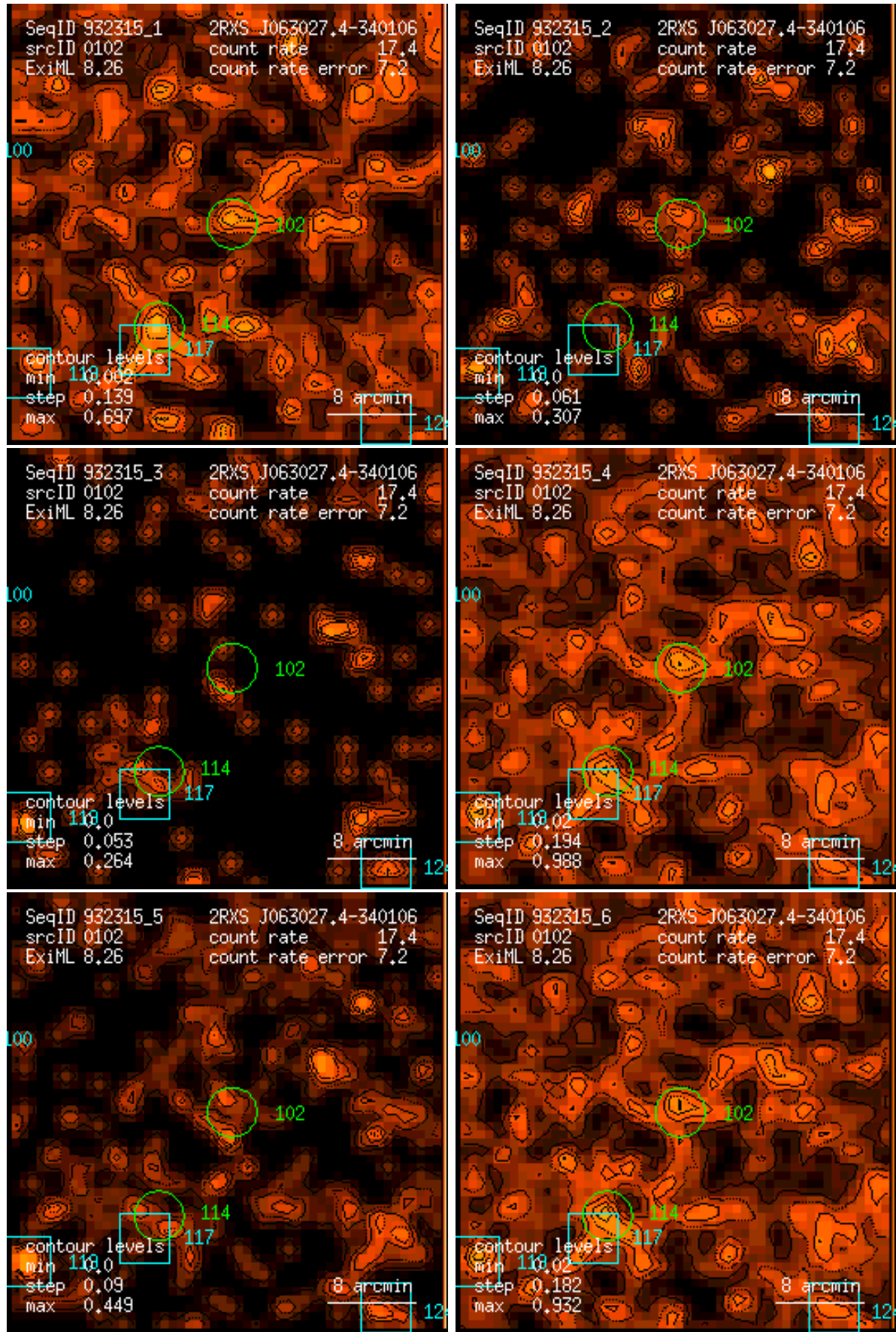
Figure 102: RASS 932315: detection 0102: band rate images, Gaussian filter: (1) PSPC channels 11 – 41, (2) 52 – 90, (3) 91 – 201, (4) 11 – 235, (5) 52 – 201, (6) 11 – 201. Broad band rates in counts/ks. Band rate contour levels in counts/ks/arcmin 2 .
