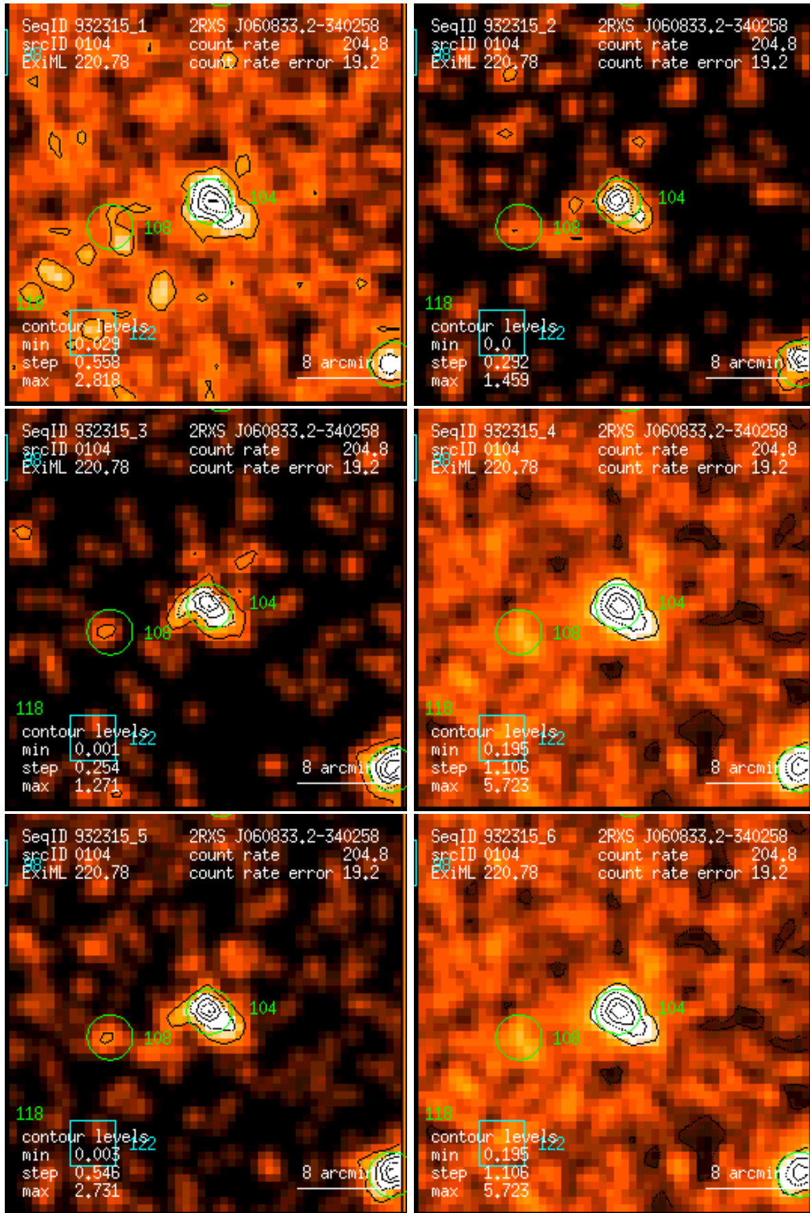
Figure 104: RASS 932315: detection 0104: band rate images, Gaussian filter: (1) PSPC channels 11 – 41, (2) 52 – 90, (3) 91 – 201, (4) 11 – 235, (5) 52 – 201, (6) 11 – 201. Broad band rates in counts/ks. Band rate contour levels in counts/ks/arcmin 2 .
