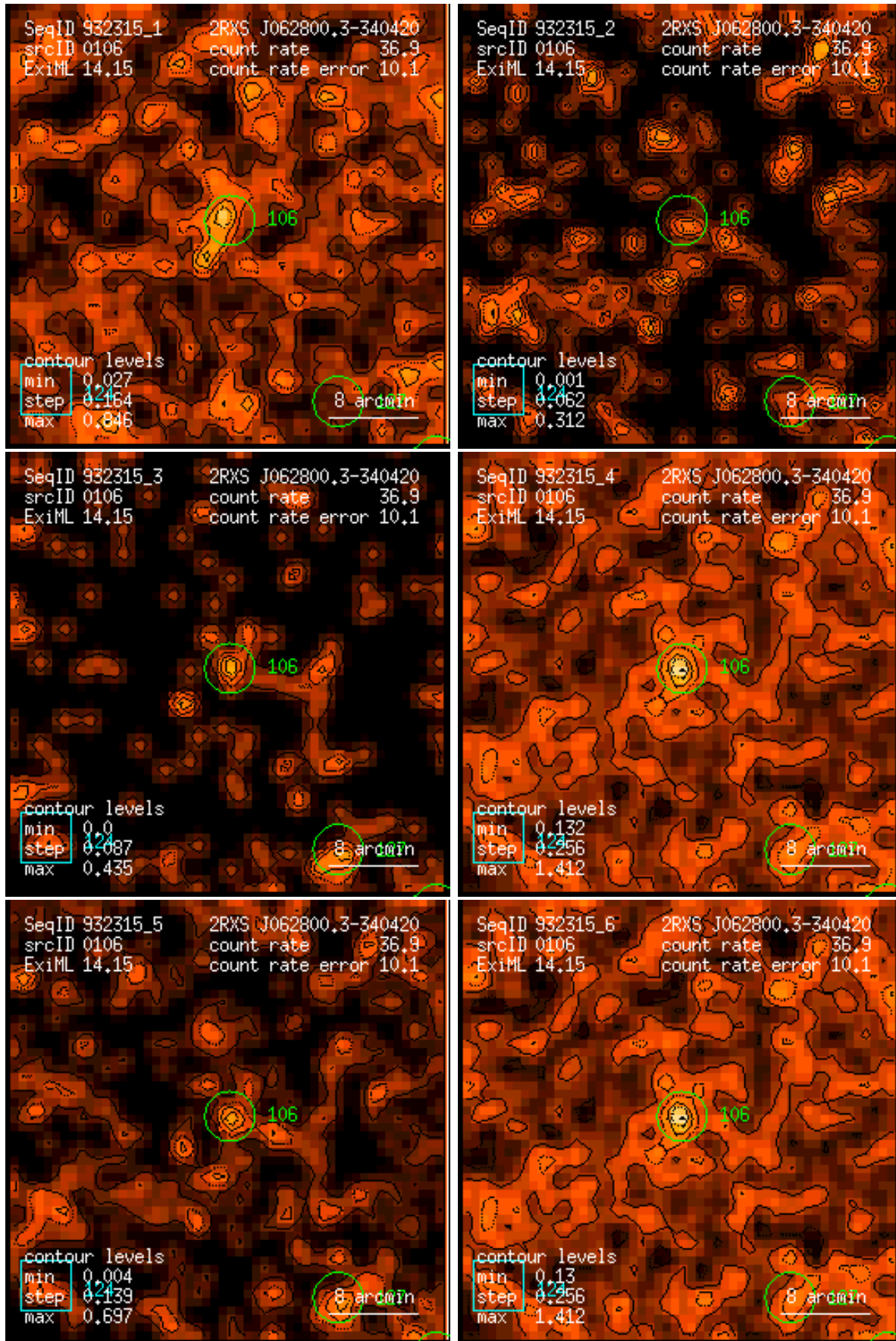
Figure 106: RASS 932315: detection 0106: band rate images, Gaussian filter: (1) PSPC channels 11 – 41, (2) 52 – 90, (3) 91 – 201, (4) 11 – 235, (5) 52 – 201, (6) 11 – 201. Broad band rates in counts/ks. Band rate contour levels in counts/ks/arcmin 2 .
