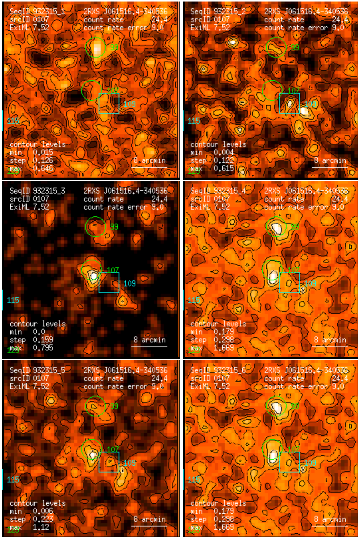
Figure 107: RASS 932315: detection 0107: band rate images, Gaussian filter: (1) PSPC channels 11 – 41, (2) 52 – 90, (3) 91 – 201, (4) 11 – 235, (5) 52 – 201, (6) 11 – 201. Broad band rates in counts/ks. Band rate contour levels in counts/ks/arcmin 2 .
