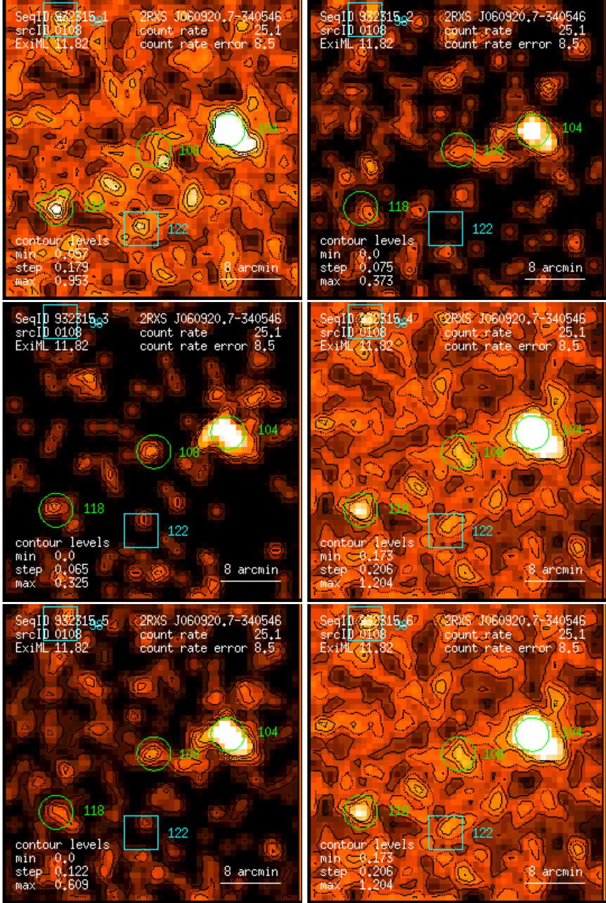
Figure 108: RASS 932315: detection 0108: band rate images, Gaussian filter: (1) PSPC channels 11 – 41, (2) 52 – 90, (3) 91 – 201, (4) 11 – 235, (5) 52 – 201, (6) 11 – 201. Broad band rates in counts/ks. Band rate contour levels in counts/ks/arcmin 2 .
