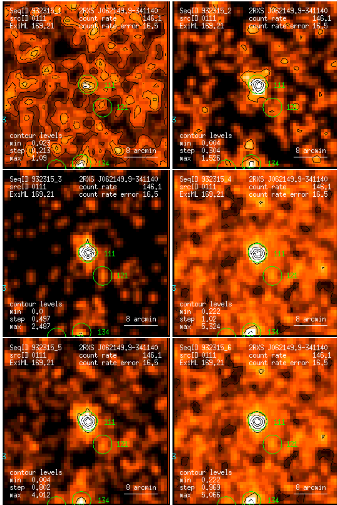
Figure 111: RASS 932315: detection 0111: band rate images, Gaussian filter: (1) PSPC channels 11 – 41, (2) 52 – 90, (3) 91 – 201, (4) 11 – 235, (5) 52 – 201, (6) 11 – 201. Broad band rates in counts/ks. Band rate contour levels in counts/ks/arcmin 2 .
