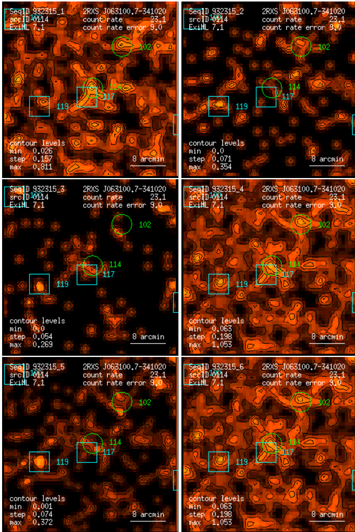
Figure 114: RASS 932315: detection 0114: band rate images, Gaussian filter: (1) PSPC channels 11 – 41, (2) 52 – 90, (3) 91 – 201, (4) 11 – 235, (5) 52 – 201, (6) 11 – 201. Broad band rates in counts/ks. Band rate contour levels in counts/ks/arcmin 2 .
