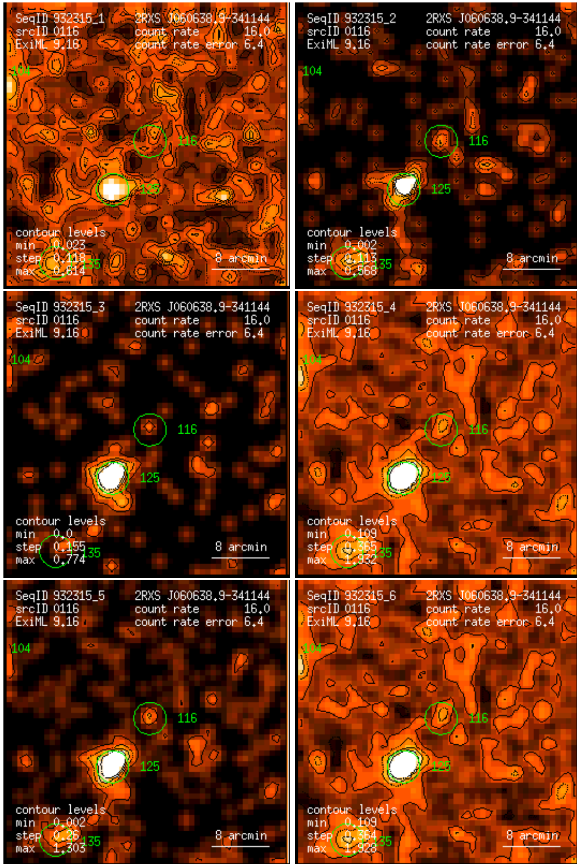
Figure 116: RASS 932315: detection 0116: band rate images, Gaussian filter: (1) PSPC channels 11 – 41, (2) 52 – 90, (3) 91 – 201, (4) 11 – 235, (5) 52 – 201, (6) 11 – 201. Broad band rates in counts/ks. Band rate contour levels in counts/ks/arcmin 2 .
