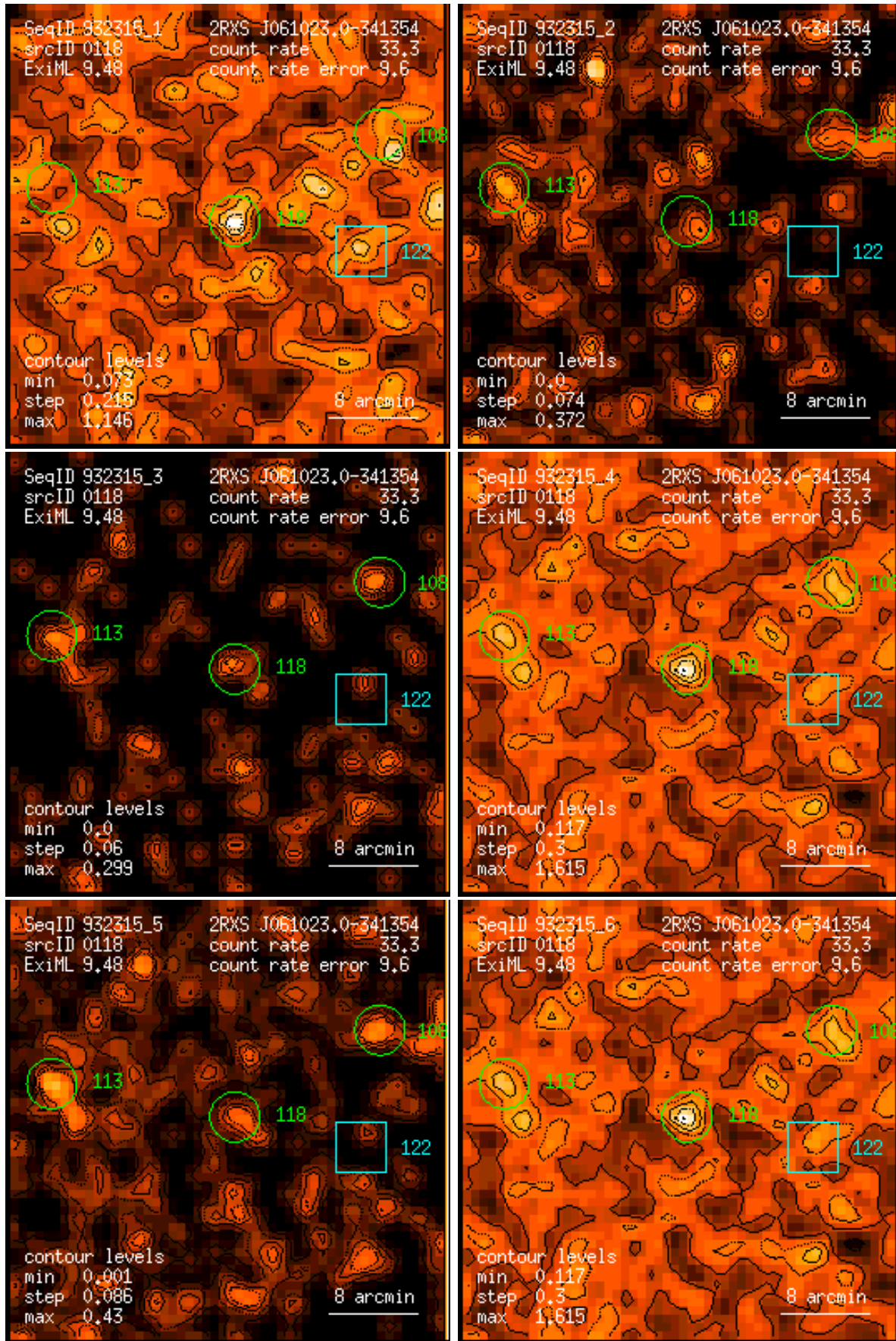
Figure 118: RASS 932315: detection 0118: band rate images, Gaussian filter: (1) PSPC channels 11 – 41, (2) 52 – 90, (3) 91 – 201, (4) 11 – 235, (5) 52 – 201, (6) 11 – 201. Broad band rates in counts/ks. Band rate contour levels in counts/ks/arcmin 2 .
