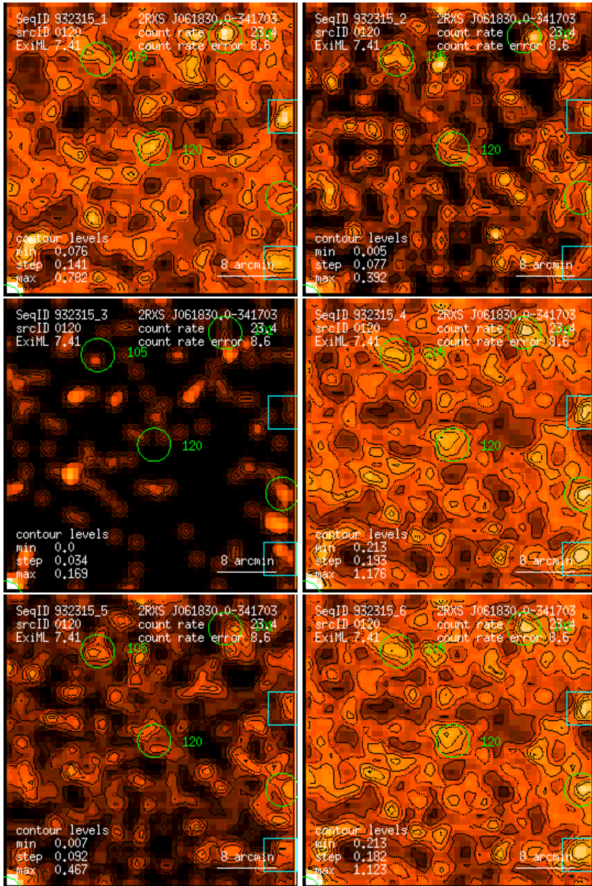
Figure 120: RASS 932315: detection 0120: band rate images, Gaussian filter: (1) PSPC channels 11 – 41, (2) 52 – 90, (3) 91 – 201, (4) 11 – 235, (5) 52 – 201, (6) 11 – 201. Broad band rates in counts/ks. Band rate contour levels in counts/ks/arcmin 2 .
