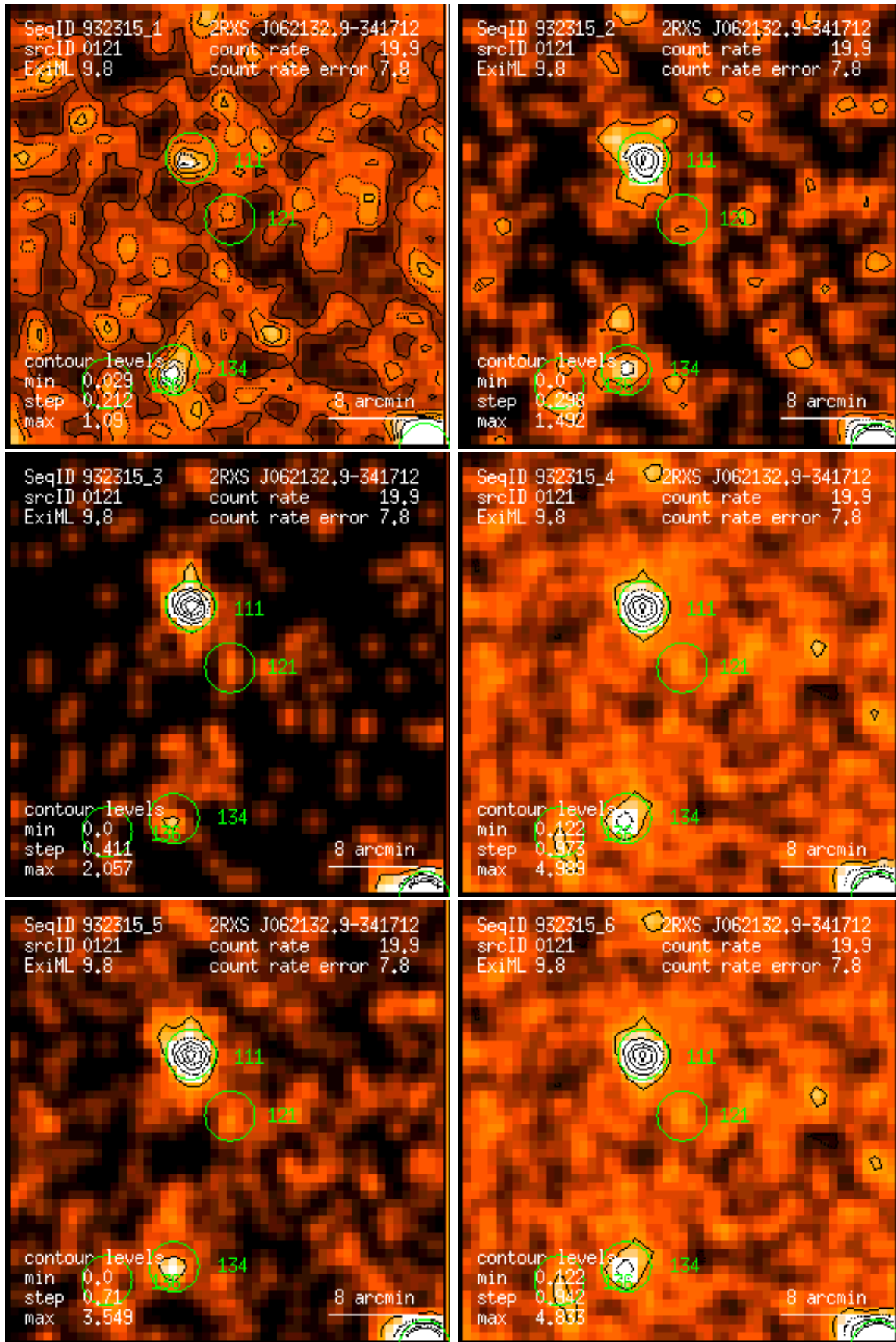
Figure 121: RASS 932315: detection 0121: band rate images, Gaussian filter: (1) PSPC channels 11 – 41, (2) 52 – 90, (3) 91 – 201, (4) 11 – 235, (5) 52 – 201, (6) 11 – 201. Broad band rates in counts/ks. Band rate contour levels in counts/ks/arcmin 2 .
