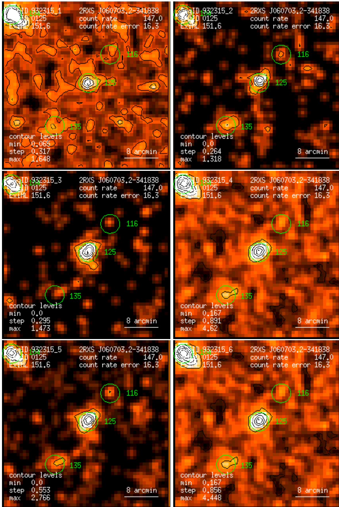
Figure 125: RASS 932315: detection 0125: band rate images, Gaussian filter: (1) PSPC channels 11 – 41, (2) 52 – 90, (3) 91 – 201, (4) 11 – 235, (5) 52 – 201, (6) 11 – 201. Broad band rates in counts/ks. Band rate contour levels in counts/ks/arcmin 2 .
