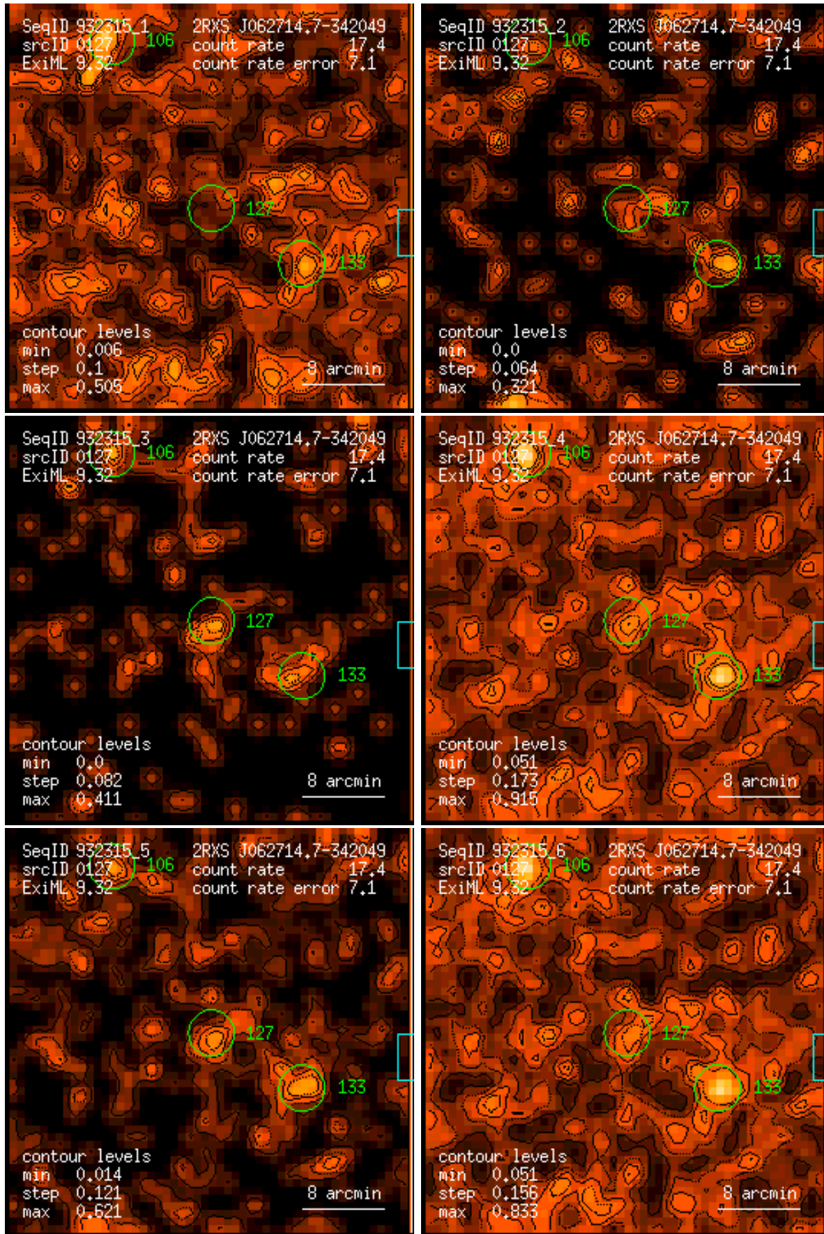
Figure 127: RASS 932315: detection 0127: band rate images, Gaussian filter: (1) PSPC channels 11 – 41, (2) 52 – 90, (3) 91 – 201, (4) 11 – 235, (5) 52 – 201, (6) 11 – 201. Broad band rates in counts/ks. Band rate contour levels in counts/ks/arcmin 2 .
