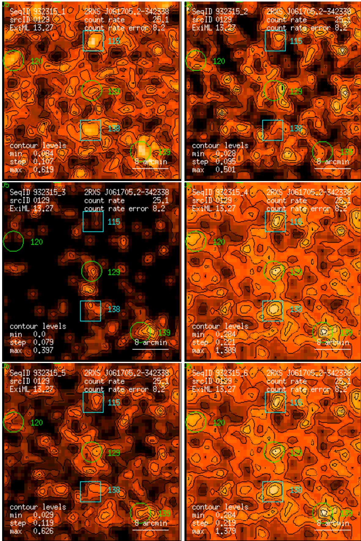
Figure 129: RASS 932315: detection 0129: band rate images, Gaussian filter: (1) PSPC channels 11 – 41, (2) 52 – 90, (3) 91 – 201, (4) 11 – 235, (5) 52 – 201, (6) 11 – 201. Broad band rates in counts/ks. Band rate contour levels in counts/ks/arcmin 2 .
