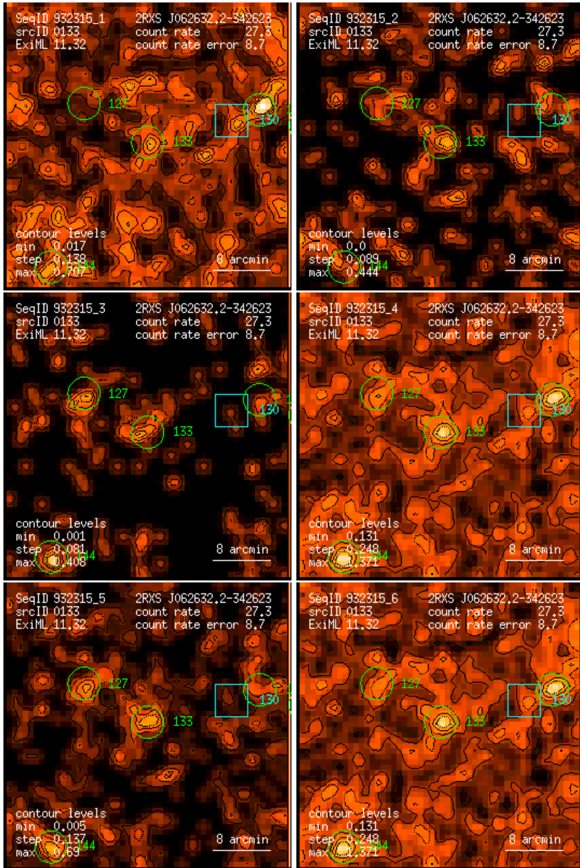
Figure 133: RASS 932315: detection 0133: band rate images, Gaussian filter: (1) PSPC channels 11 – 41, (2) 52 – 90, (3) 91 – 201, (4) 11 – 235, (5) 52 – 201, (6) 11 – 201. Broad band rates in counts/ks. Band rate contour levels in counts/ks/arcmin 2 .
