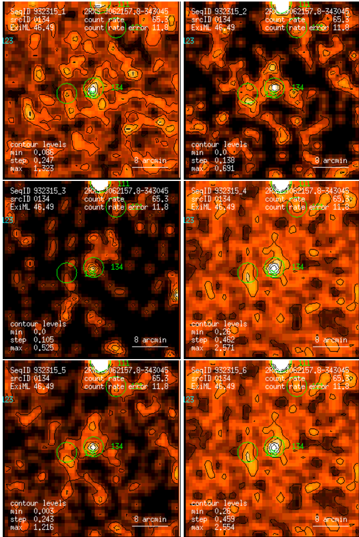
Figure 134: RASS 932315: detection 0134: band rate images, Gaussian filter: (1) PSPC channels 11 – 41, (2) 52 – 90, (3) 91 – 201, (4) 11 – 235, (5) 52 – 201, (6) 11 – 201. Broad band rates in counts/ks. Band rate contour levels in counts/ks/arcmin 2 .
