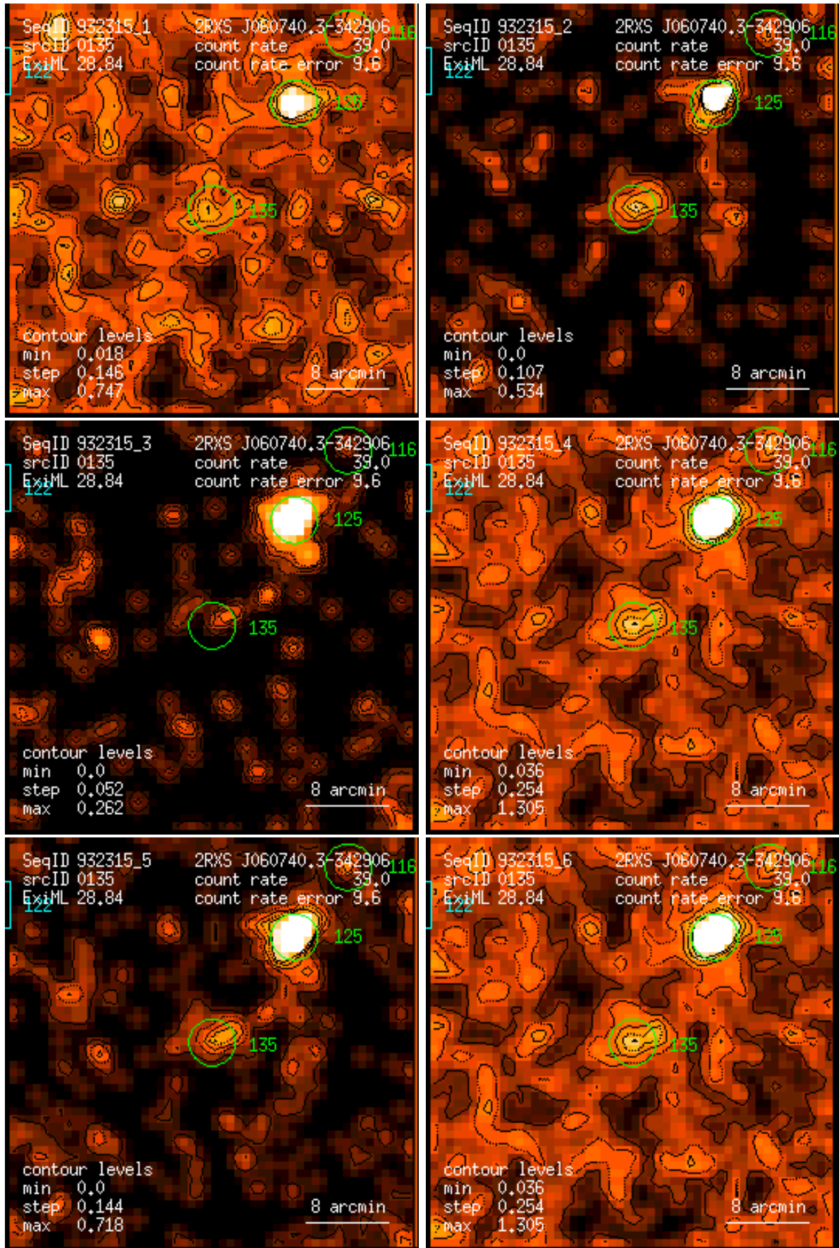
Figure 135: RASS 932315: detection 0135: band rate images, Gaussian filter: (1) PSPC channels 11 – 41, (2) 52 – 90, (3) 91 – 201, (4) 11 – 235, (5) 52 – 201, (6) 11 – 201. Broad band rates in counts/ks. Band rate contour levels in counts/ks/arcmin 2 .
