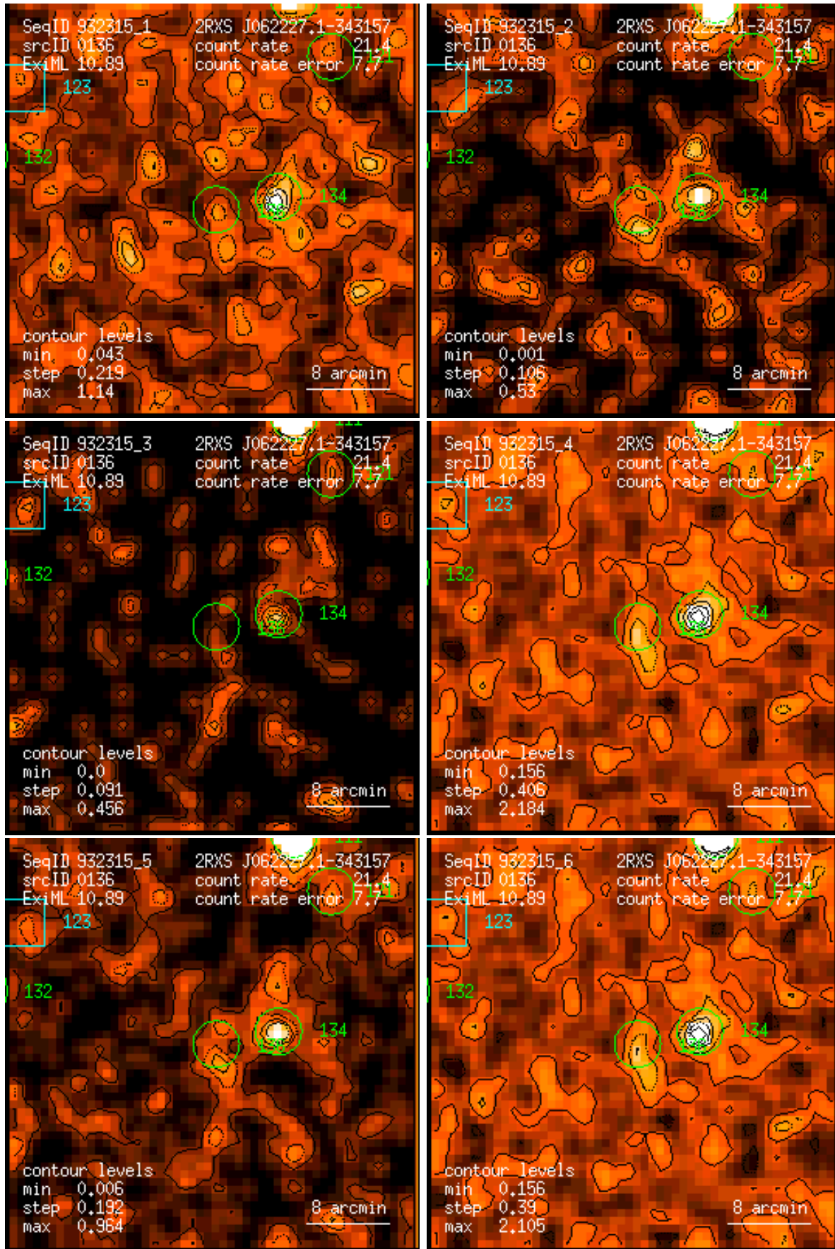
Figure 136: RASS 932315: detection 0136: band rate images, Gaussian filter: (1) PSPC channels 11 – 41, (2) 52 – 90, (3) 91 – 201, (4) 11 – 235, (5) 52 – 201, (6) 11 – 201. Broad band rates in counts/ks. Band rate contour levels in counts/ks/arcmin 2 .
