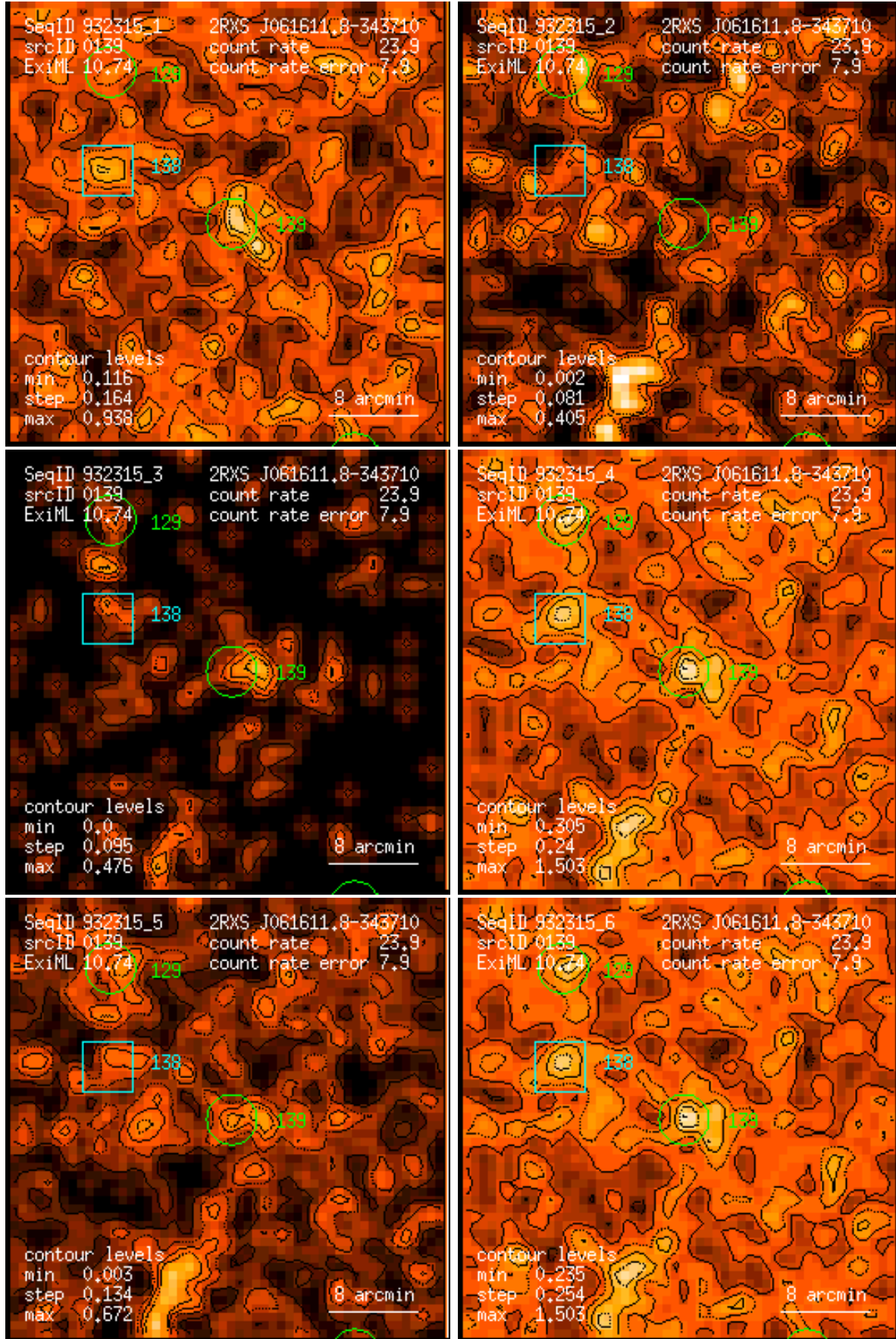
Figure 139: RASS 932315: detection 0139: band rate images, Gaussian filter: (1) PSPC channels 11 – 41, (2) 52 – 90, (3) 91 – 201, (4) 11 – 235, (5) 52 – 201, (6) 11 – 201. Broad band rates in counts/ks. Band rate contour levels in counts/ks/arcmin 2 .
