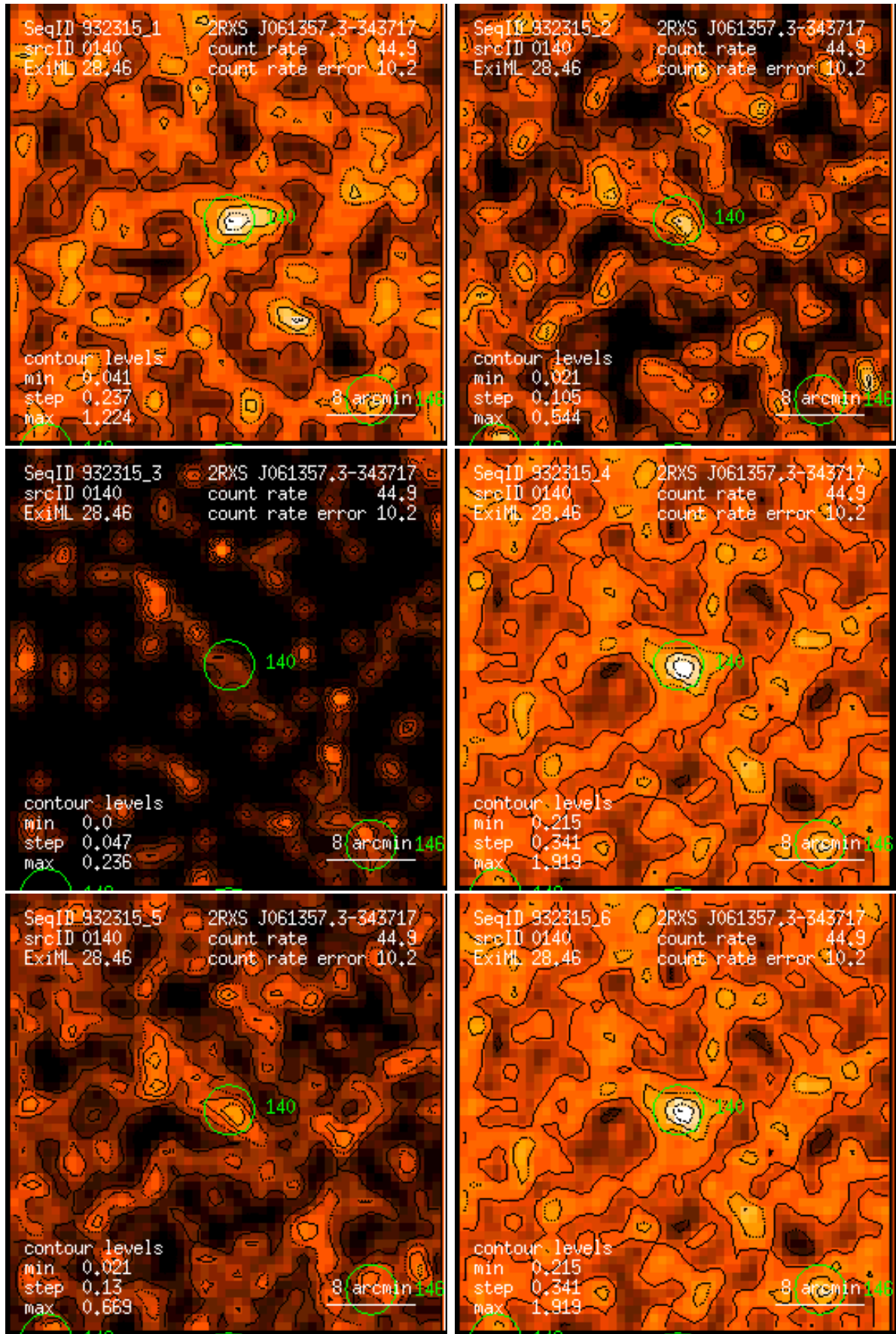
Figure 140: RASS 932315: detection 0140: band rate images, Gaussian filter: (1) PSPC channels 11 – 41, (2) 52 – 90, (3) 91 – 201, (4) 11 – 235, (5) 52 – 201, (6) 11 – 201. Broad band rates in counts/ks. Band rate contour levels in counts/ks/arcmin 2 .
