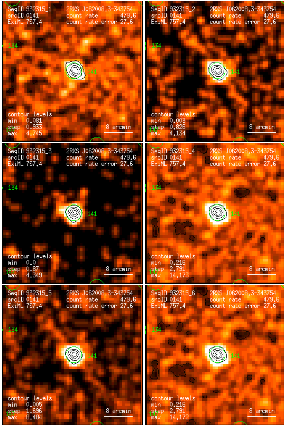
Figure 141: RASS 932315: detection 0141: band rate images, Gaussian filter: (1) PSPC channels 11 – 41, (2) 52 – 90, (3) 91 – 201, (4) 11 – 235, (5) 52 – 201, (6) 11 – 201. Broad band rates in counts/ks. Band rate contour levels in counts/ks/arcmin 2 .
