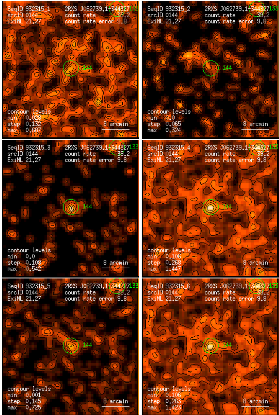
Figure 144: RASS 932315: detection 0144: band rate images, Gaussian filter: (1) PSPC channels 11 – 41, (2) 52 – 90, (3) 91 – 201, (4) 11 – 235, (5) 52 – 201, (6) 11 – 201. Broad band rates in counts/ks. Band rate contour levels in counts/ks/arcmin 2 .
