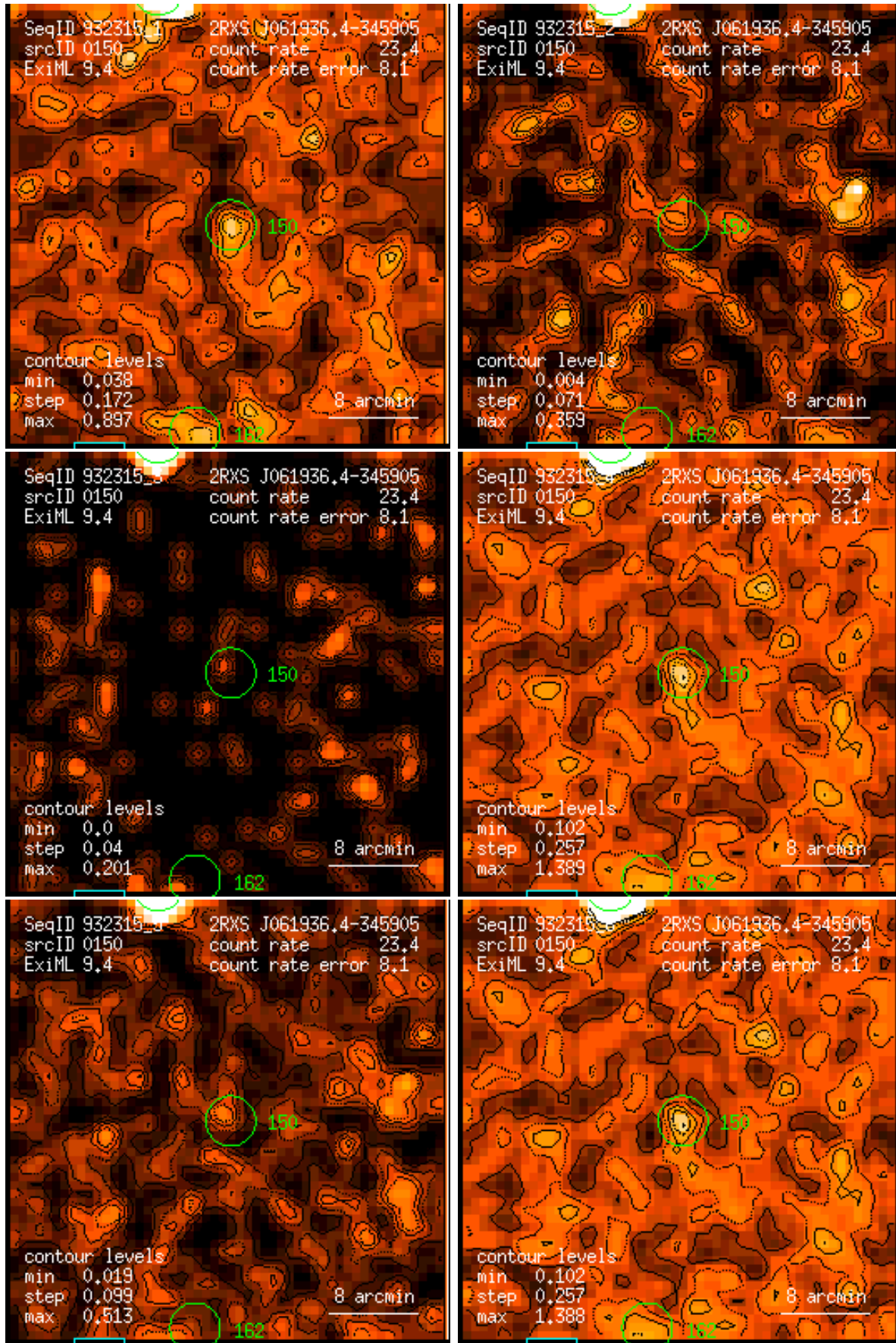
Figure 150: RASS 932315: detection 0150: band rate images, Gaussian filter: (1) PSPC channels 11 – 41, (2) 52 – 90, (3) 91 – 201, (4) 11 – 235, (5) 52 – 201, (6) 11 – 201. Broad band rates in counts/ks. Band rate contour levels in counts/ks/arcmin 2 .
