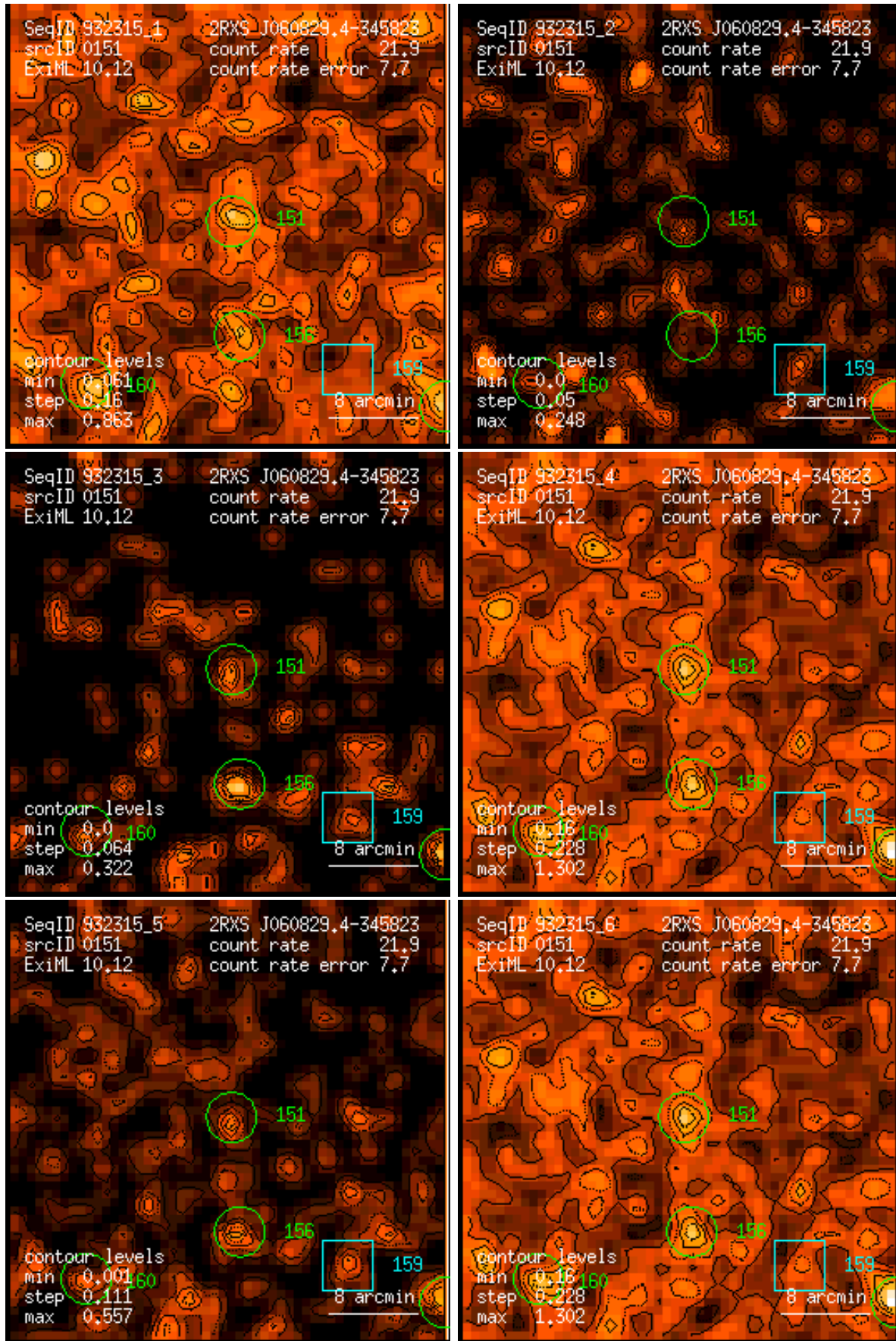
Figure 151: RASS 932315: detection 0151: band rate images, Gaussian filter: (1) PSPC channels 11 – 41, (2) 52 – 90, (3) 91 – 201, (4) 11 – 235, (5) 52 – 201, (6) 11 – 201. Broad band rates in counts/ks. Band rate contour levels in counts/ks/arcmin 2 .
