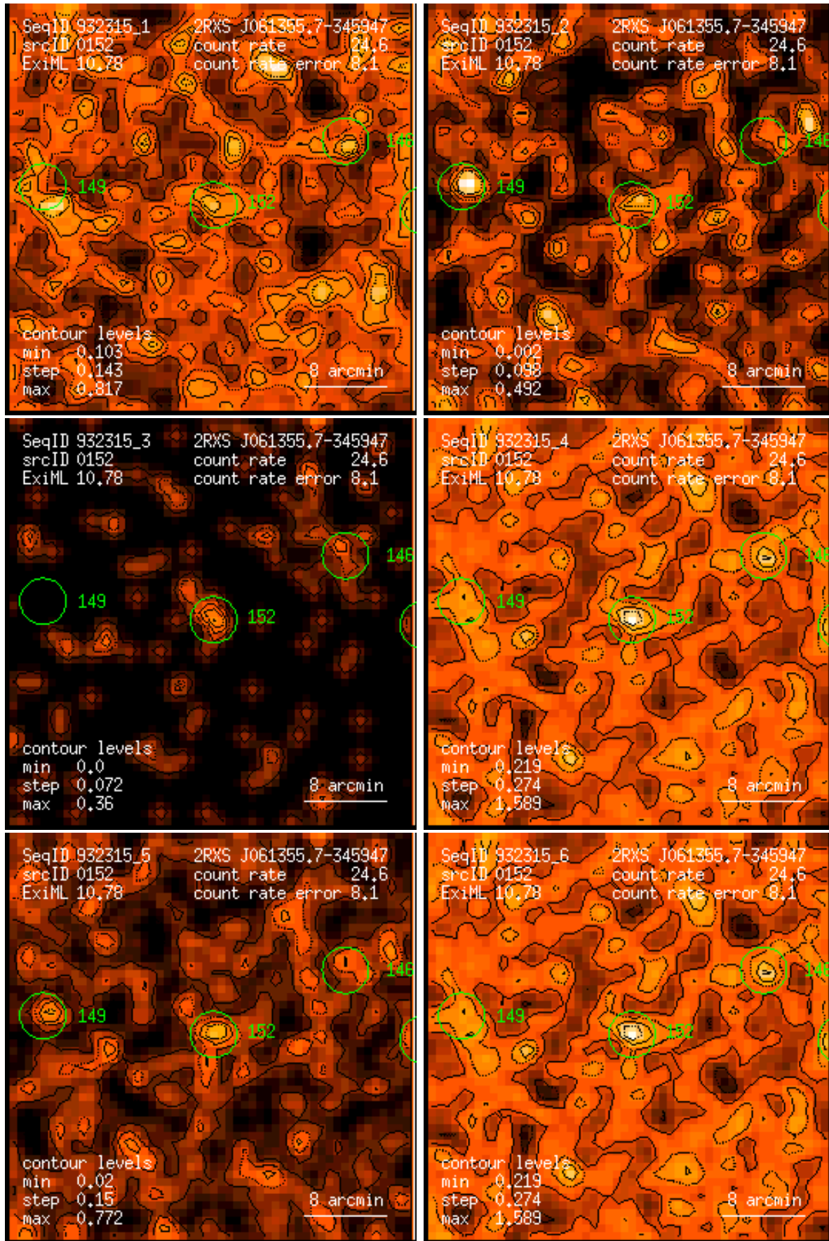
Figure 152: RASS 932315: detection 0152: band rate images, Gaussian filter: (1) PSPC channels 11 – 41, (2) 52 – 90, (3) 91 – 201, (4) 11 – 235, (5) 52 – 201, (6) 11 – 201. Broad band rates in counts/ks. Band rate contour levels in counts/ks/arcmin 2 .
