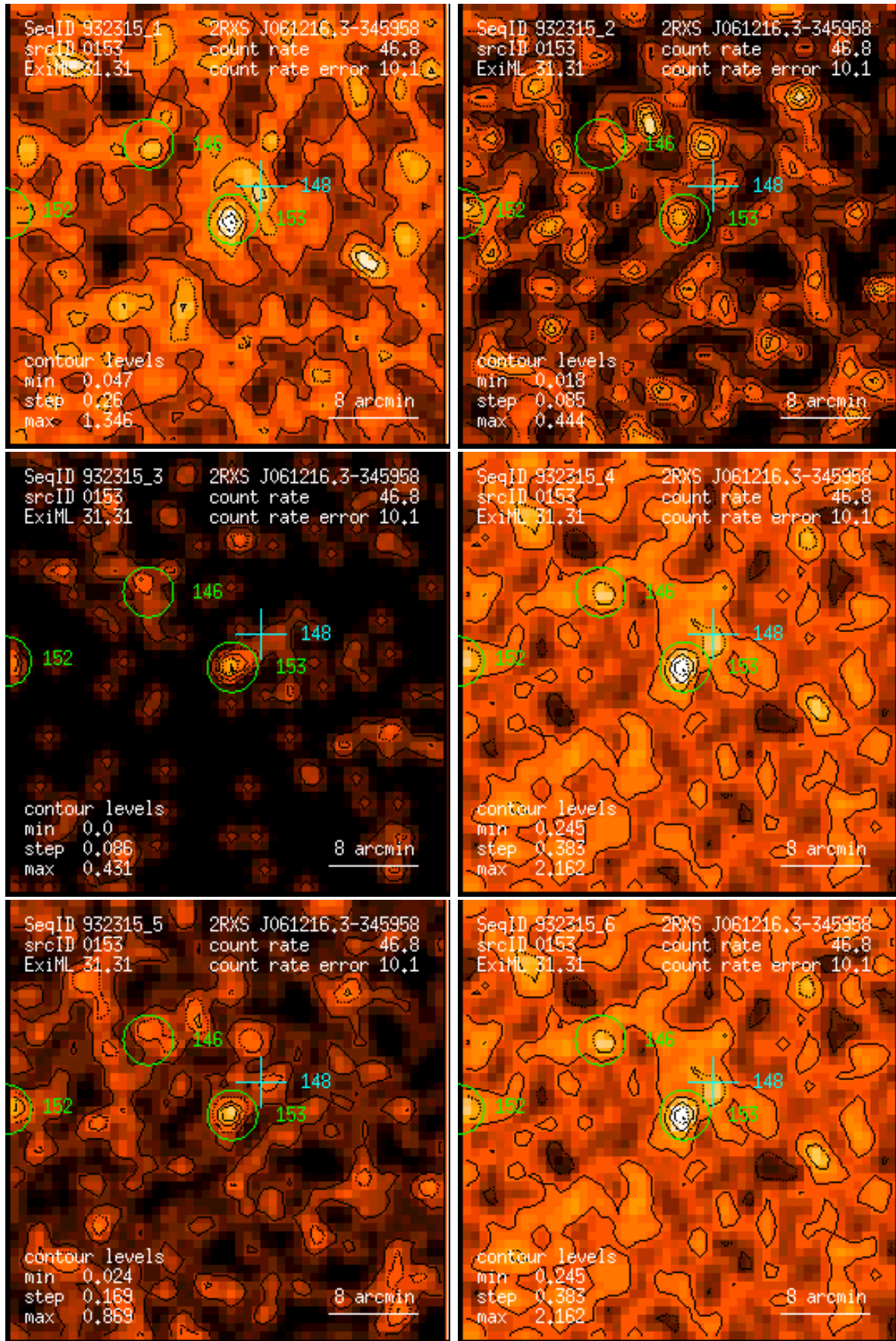
Figure 153: RASS 932315: detection 0153: band rate images, Gaussian filter: (1) PSPC channels 11 – 41, (2) 52 – 90, (3) 91 – 201, (4) 11 – 235, (5) 52 – 201, (6) 11 – 201. Broad band rates in counts/ks. Band rate contour levels in counts/ks/arcmin 2 .
