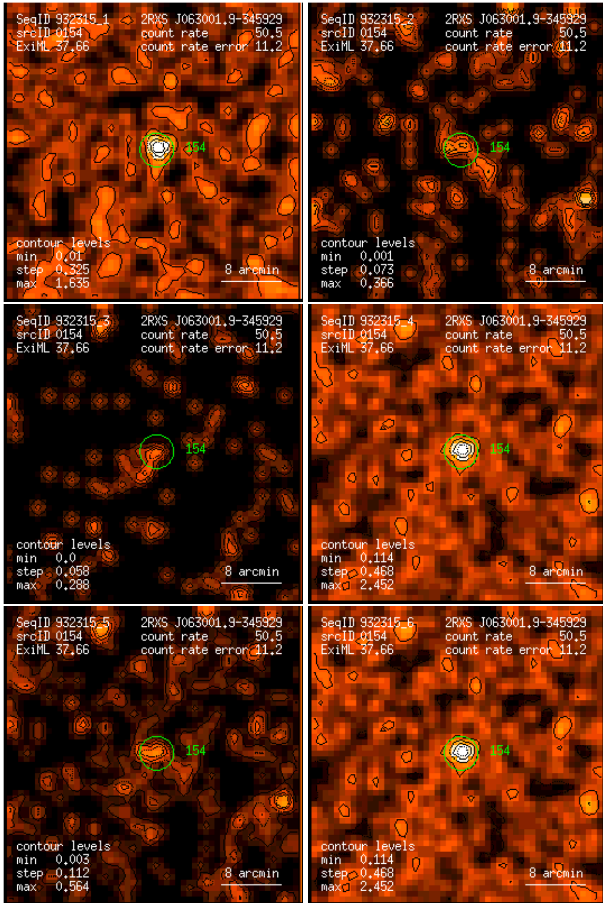
Figure 154: RASS 932315: detection 0154: band rate images, Gaussian filter: (1) PSPPC channels 11 – 41, (2) 52 – 90, (3) 91 – 201, (4) 11 – 235, (5) 52 – 201, (6) 11 – 201. Broad band rates in counts/ks. Band rate contour levels in counts/ks/arcmin 2 .
