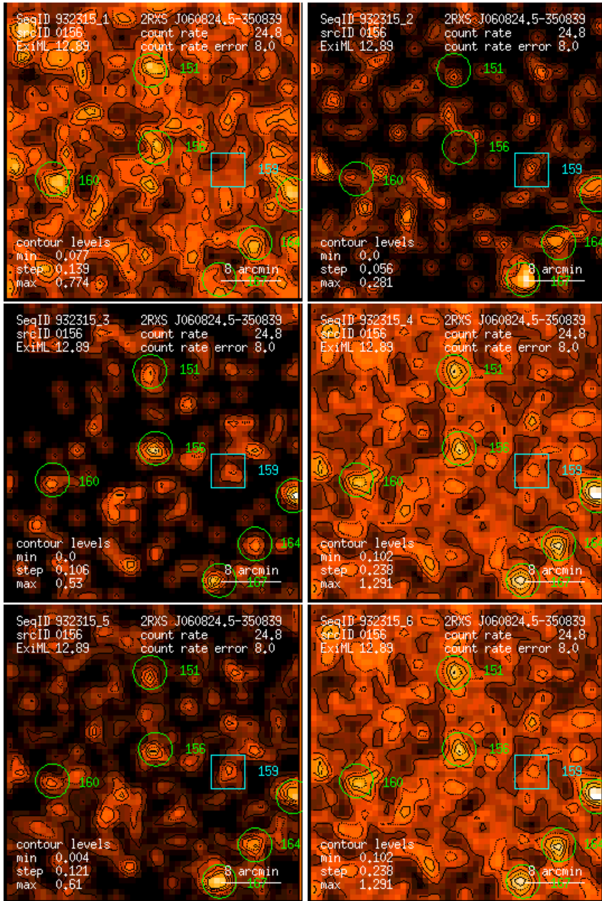
Figure 156: RASS 932315: detection 0156: band rate images, Gaussian filter: (1) PSPC channels 11 – 41, (2) 52 – 90, (3) 91 – 201, (4) 11 – 235, (5) 52 – 201, (6) 11 – 201. Broad band rates in counts/ks. Band rate contour levels in counts/ks/arcmin 2 .
