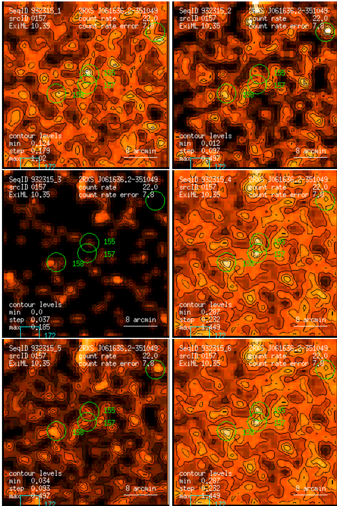
Figure 157: RASS 932315: detection 0157: band rate images, Gaussian filter: (1) PSPC channels 11 – 41, (2) 52 – 90, (3) 91 – 201, (4) 11 – 235, (5) 52 – 201, (6) 11 – 201. Broad band rates in counts/ks. Band rate contour levels in counts/ks/arcmin 2 .
