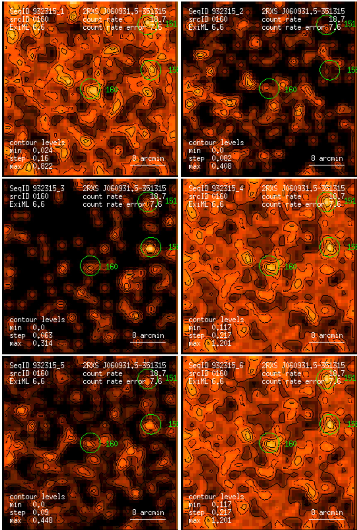
Figure 160: RASS 932315: detection 0160: band rate images, Gaussian filter: (1) PSPC channels 11 – 41, (2) 52 – 90, (3) 91 – 201, (4) 11 – 235, (5) 52 – 201, (6) 11 – 201. Broad band rates in counts/ks. Band rate contour levels in counts/ks/arcmin 2 .
