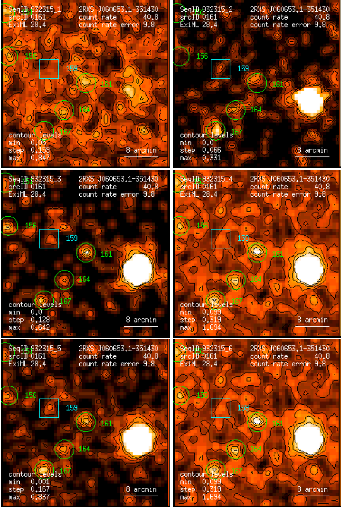
Figure 161: RASS 932315: detection 0161: band rate images, Gaussian filter: (1) PSPC channels 11 – 41, (2) 52 – 90, (3) 91 – 201, (4) 11 – 235, (5) 52 – 201, (6) 11 – 201. Broad band rates in counts/ks. Band rate contour levels in counts/ks/arcmin 2 .
