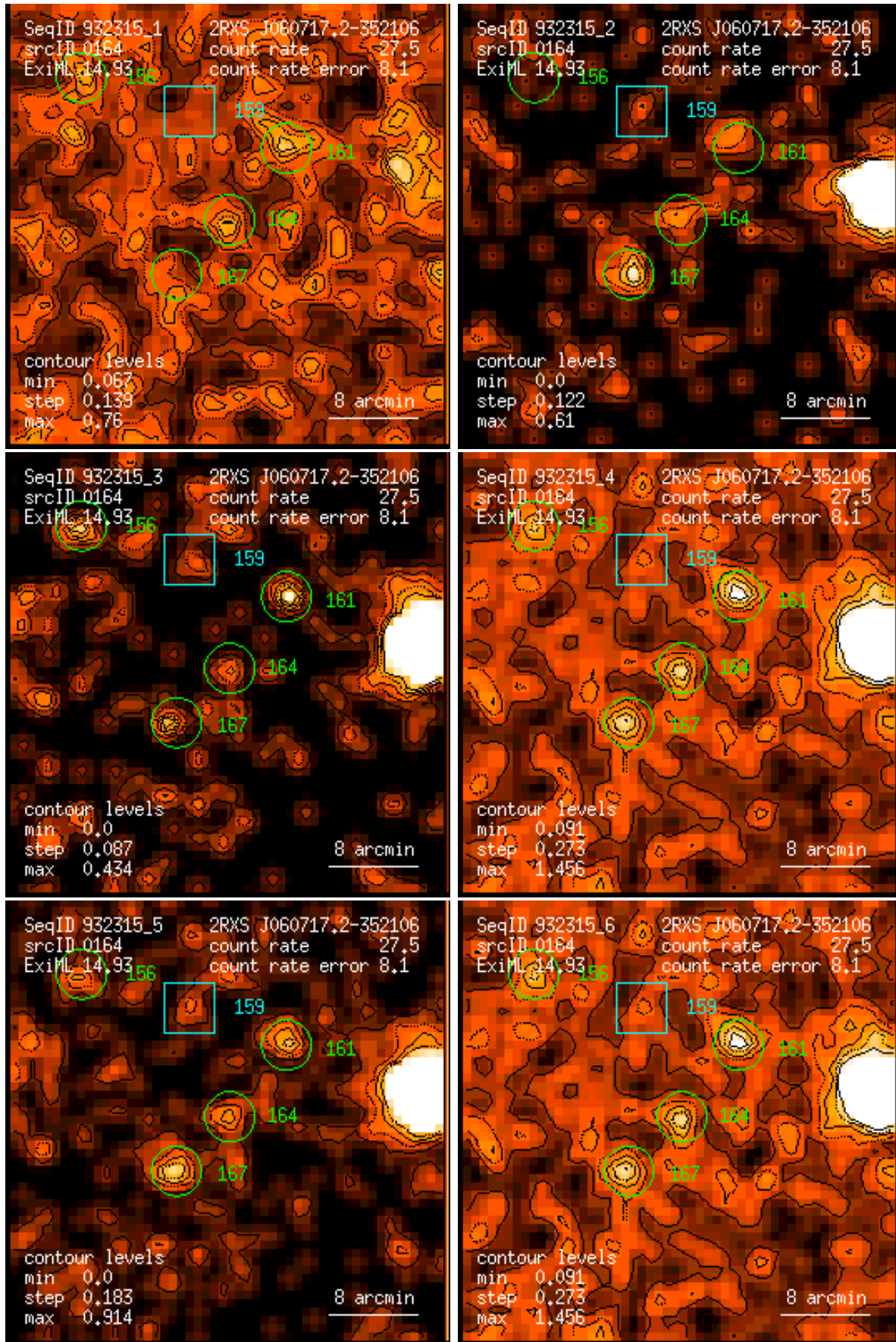
Figure 164: RASS 932315: detection 0164: band rate images, Gaussian filter: (1) PSPC channels 11 – 41, (2) 52 – 90, (3) 91 – 201, (4) 11 – 235, (5) 52 – 201, (6) 11 – 201. Broad band rates in counts/ks. Band rate contour levels in counts/ks/arcmin 2 .
