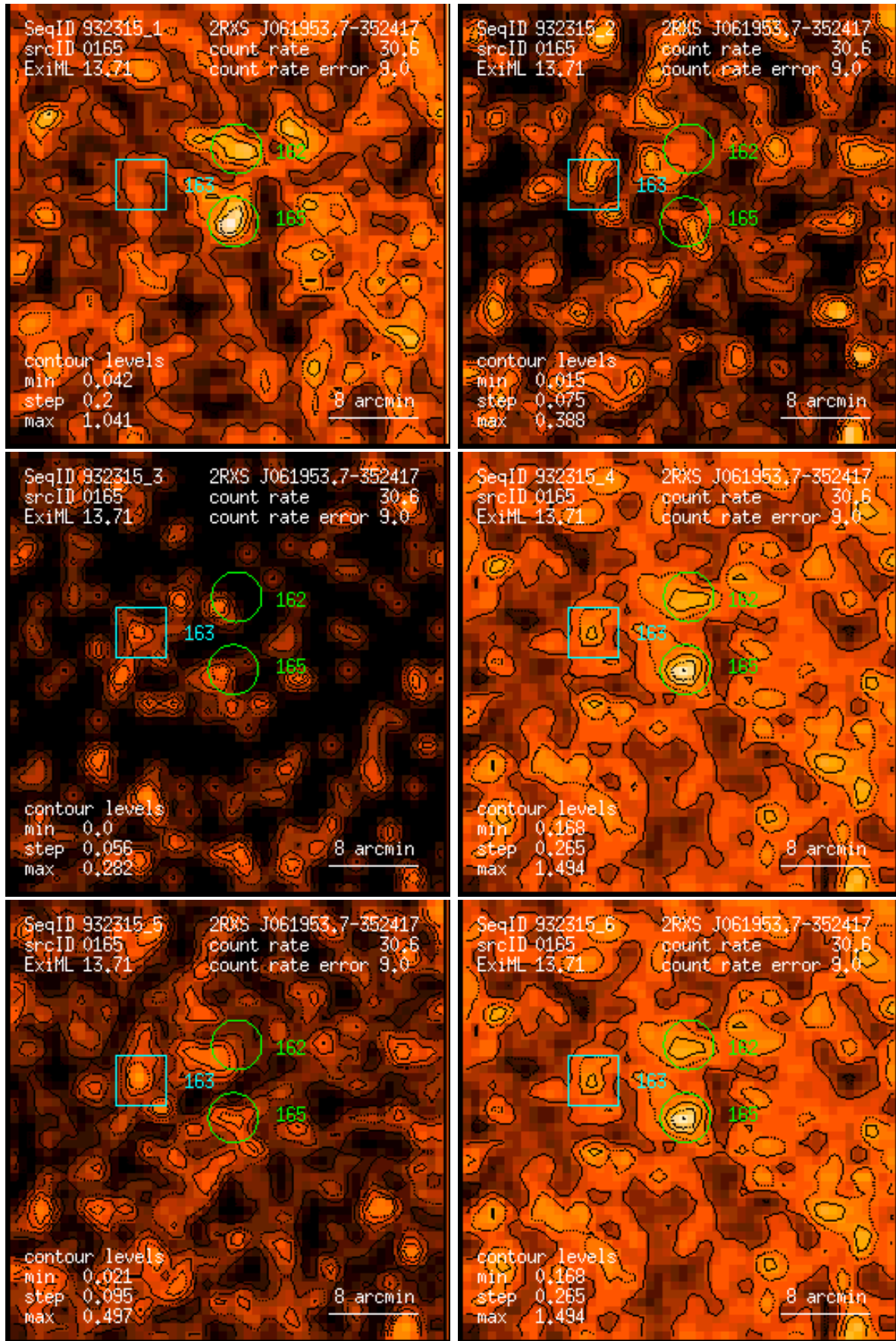
Figure 165: RASS 932315: detection 0165: band rate images, Gaussian filter: (1) PSPC channels 11 – 41, (2) 52 – 90, (3) 91 – 201, (4) 11 – 235, (5) 52 – 201, (6) 11 – 201. Broad band rates in counts/ks. Band rate contour levels in counts/ks/arcmin 2 .
