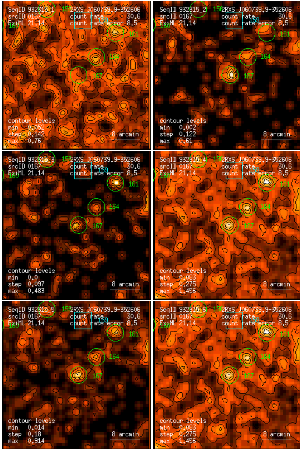
Figure 167: RASS 932315: detection 0167: band rate images, Gaussian filter: (1) PSPC channels 11 – 41, (2) 52 – 90, (3) 91 – 201, (4) 11 – 235, (5) 52 – 201, (6) 11 – 201. Broad band rates in counts/ks. Band rate contour levels in counts/ks/arcmin 2 .
