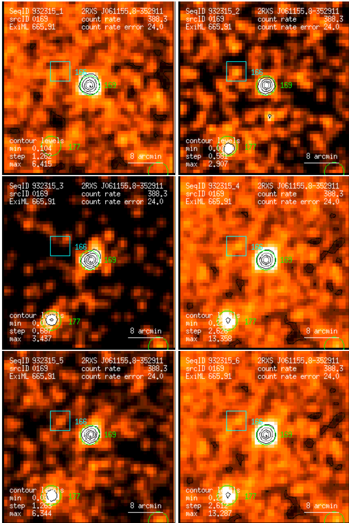
Figure 169: RASS 932315: detection 0169: band rate images, Gaussian filter: (1) PSPC channels 11 – 41, (2) 52 – 90, (3) 91 – 201, (4) 11 – 235, (5) 52 – 201, (6) 11 – 201. Broad band rates in counts/ks. Band rate contour levels in counts/ks/arcmin 2 .
