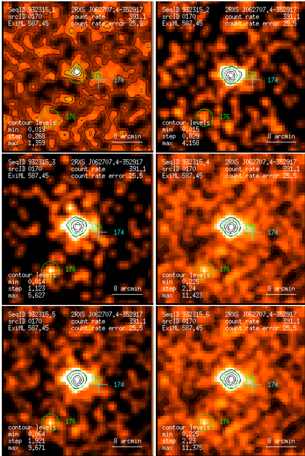
Figure 170: RASS 932315: detection 0170: band rate images, Gaussian filter: (1) PSPC channels 11 – 41, (2) 52 – 90, (3) 91 – 201, (4) 11 – 235, (5) 52 – 201, (6) 11 – 201. Broad band rates in counts/ks. Band rate contour levels in counts/ks/arcmin 2 .
