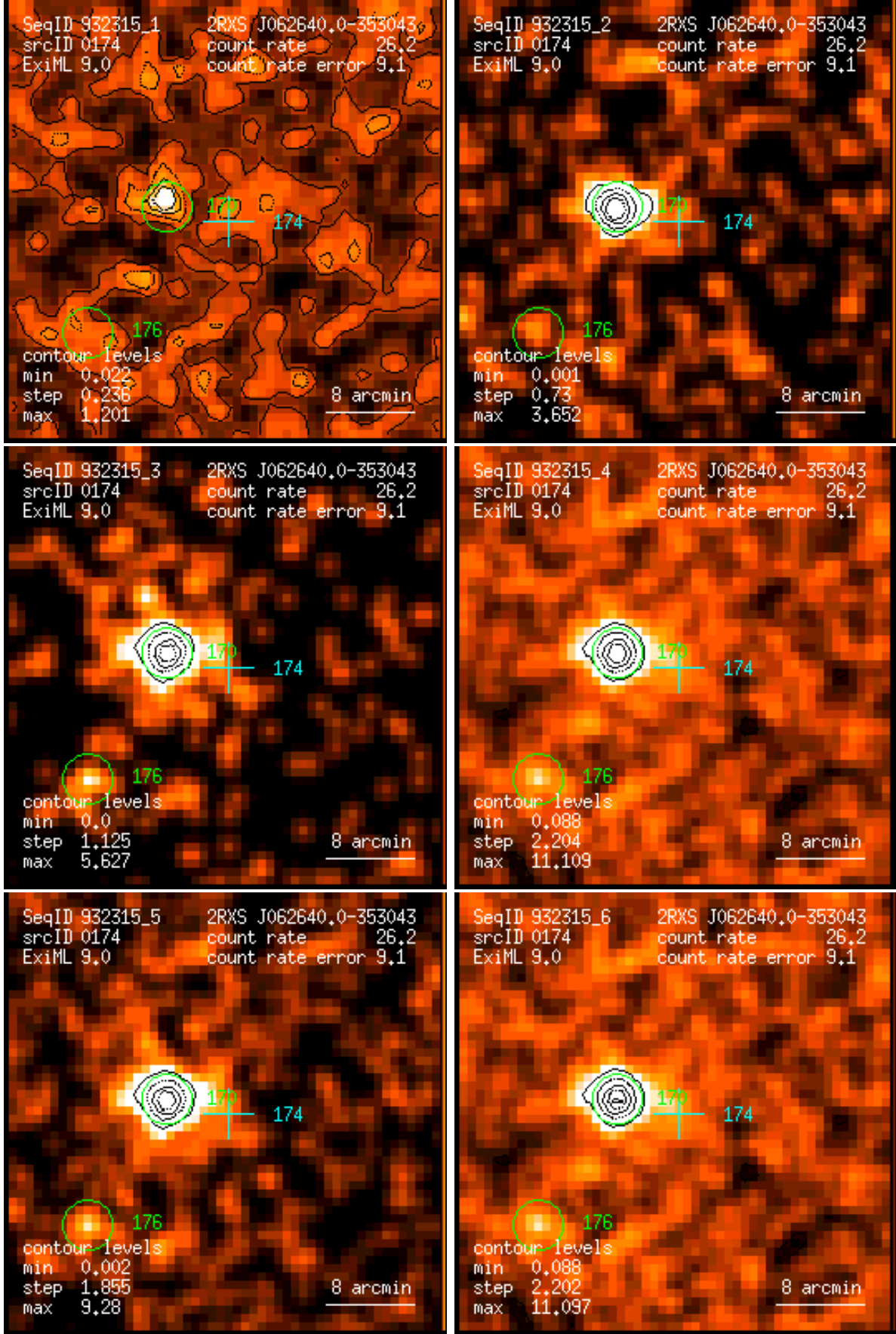
Figure 174: RASS 932315: detection 0174: band rate images, Gaussian filter: (1) PSPC channels 11 – 41, (2) 52 – 90, (3) 91 – 201, (4) 11 – 235, (5) 52 – 201, (6) 11 – 201. Broad band rates in counts/ks. Band rate contour levels in counts/ks/arcmin 2 .
