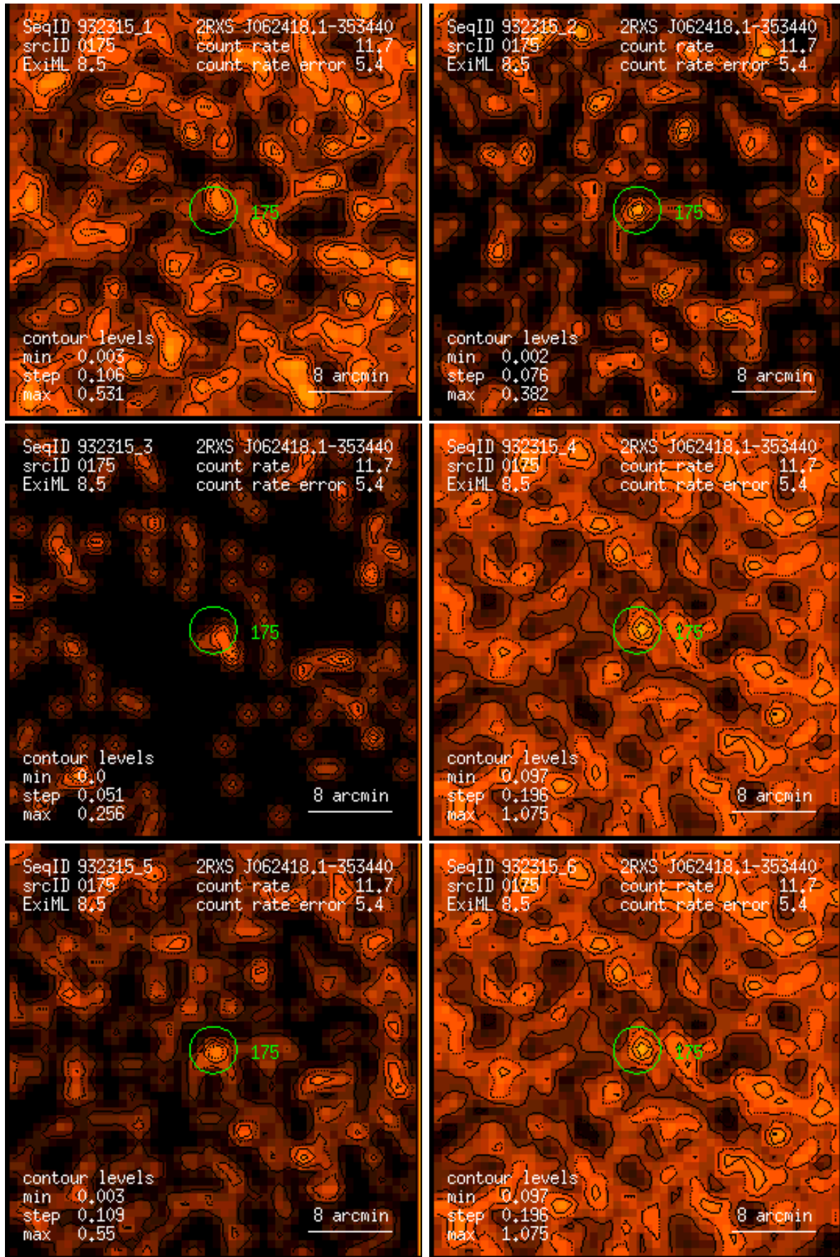
Figure 175: RASS 932315: detection 0175: band rate images, Gaussian filter: (1) PSPC channels 11 – 41, (2) 52 – 90, (3) 91 – 201, (4) 11 – 235, (5) 52 – 201, (6) 11 – 201. Broad band rates in counts/ks. Band rate contour levels in counts/ks/arcmin 2 .
