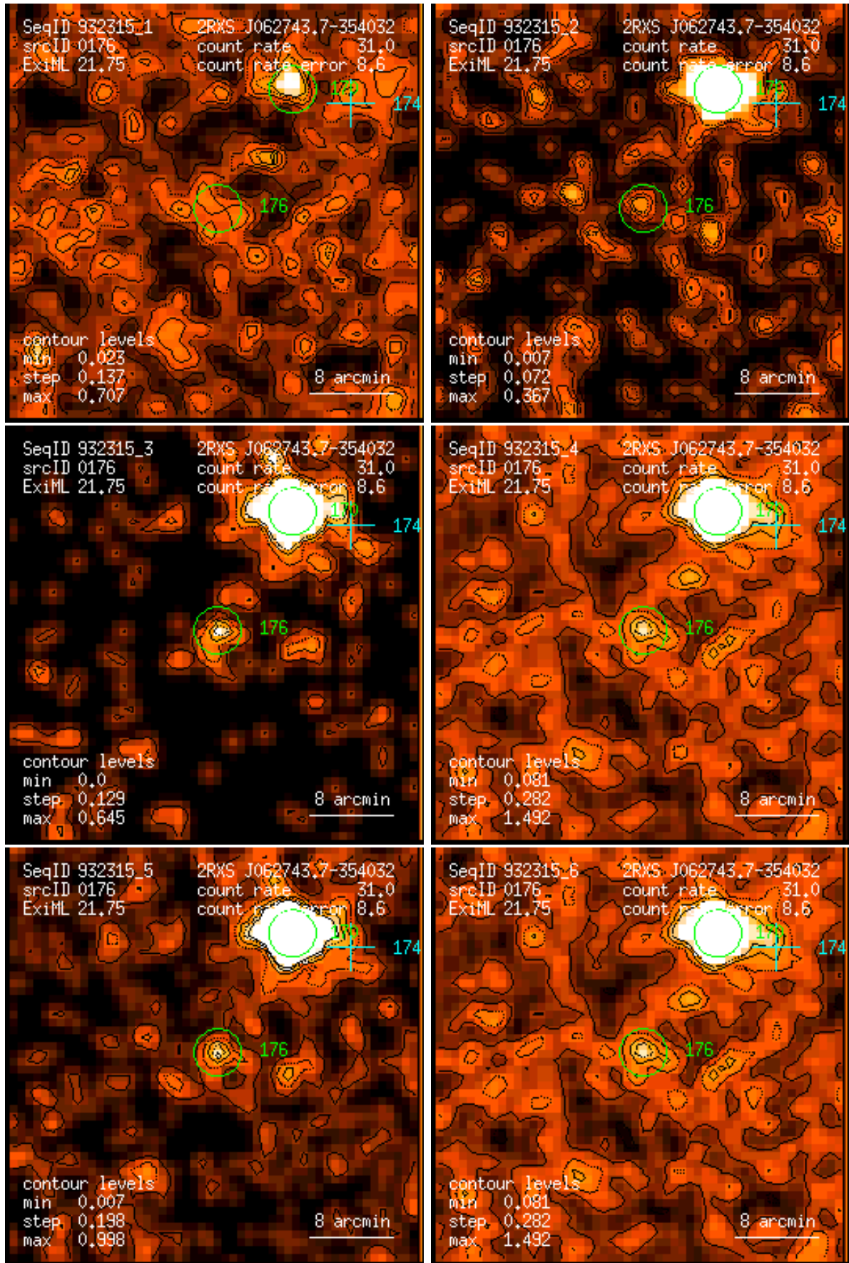
Figure 176: RASS 932315: detection 0176: band rate images, Gaussian filter: (1) PSPC channels 11 – 41, (2) 52 – 90, (3) 91 – 201, (4) 11 – 235, (5) 52 – 201, (6) 11 – 201. Broad band rates in counts/ks. Band rate contour levels in counts/ks/arcmin 2 .
