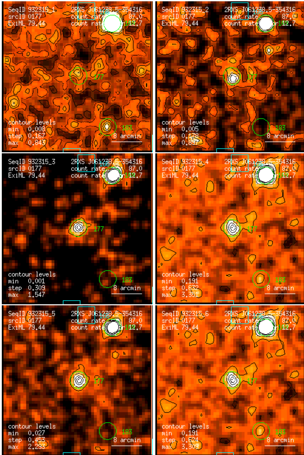
Figure 177: RASS 932315: detection 0177: band rate images, Gaussian filter: (1) PSPC channels 11 – 41, (2) 52 – 90, (3) 91 – 201, (4) 11 – 235, (5) 52 – 201, (6) 11 – 201. Broad band rates in counts/ks. Band rate contour levels in counts/ks/arcmin 2 .
