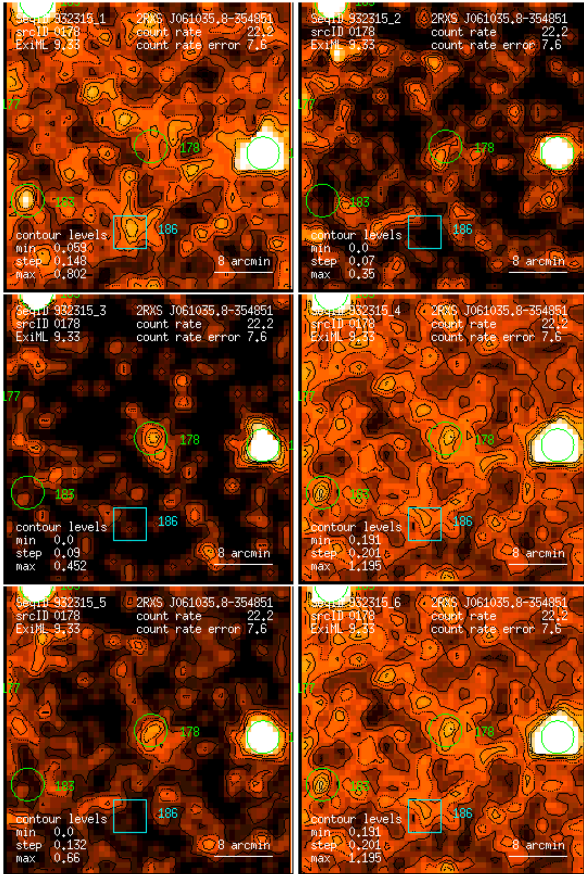
Figure 178: RASS 932315: detection 0178: band rate images, Gaussian filter: (1) PSPC channels 11 – 41, (2) 52 – 90, (3) 91 – 201, (4) 11 – 235, (5) 52 – 201, (6) 11 – 201. Broad band rates in counts/ks. Band rate contour levels in counts/ks/arcmin 2 .
