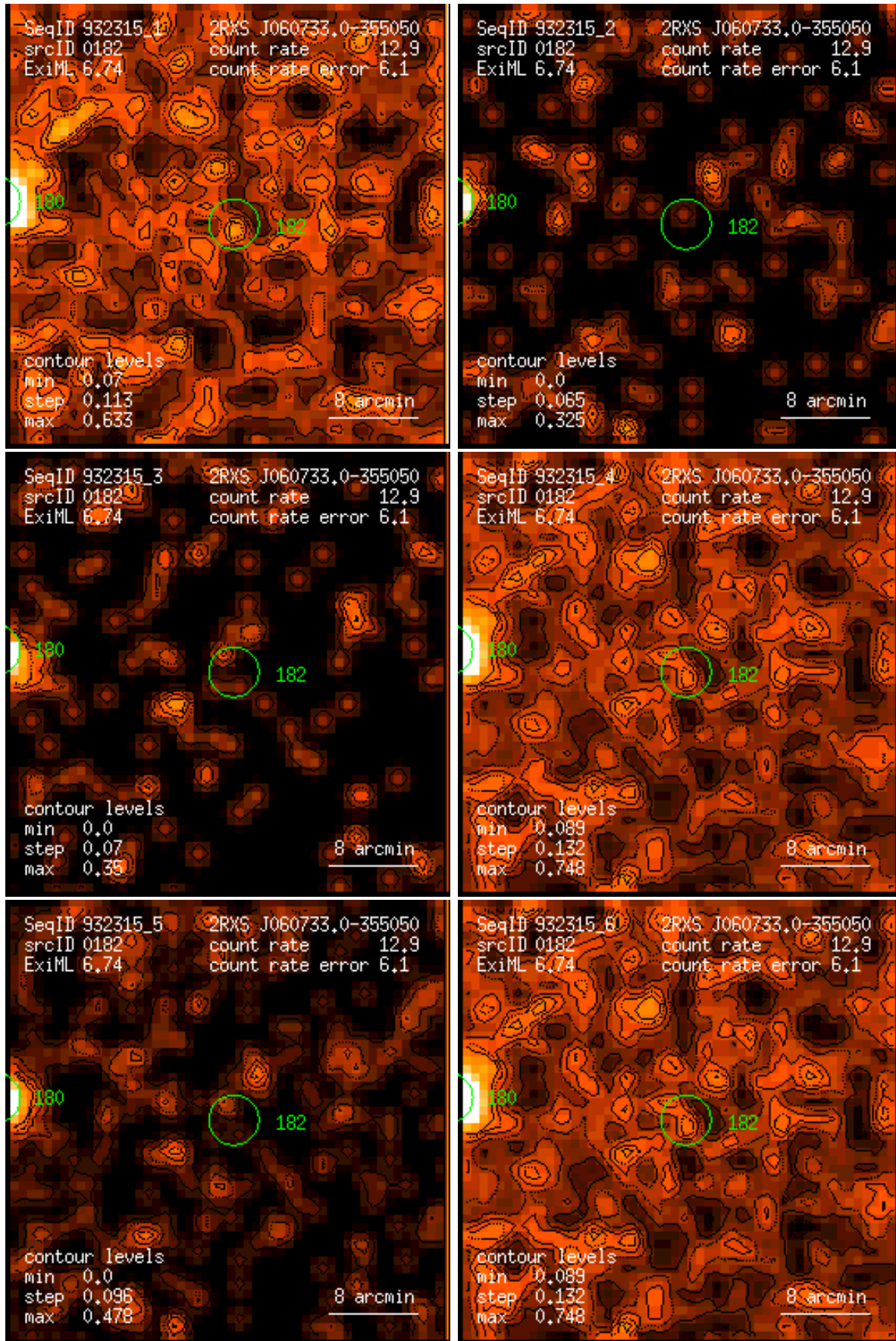
Figure 182: RASS 932315: detection 0182: band rate images, Gaussian filter: (1) PSPC channels 11 – 41, (2) 52 – 90, (3) 91 – 201, (4) 11 – 235, (5) 52 – 201, (6) 11 – 201. Broad band rates in counts/ks. Band rate contour levels in counts/ks/arcmin 2 .
