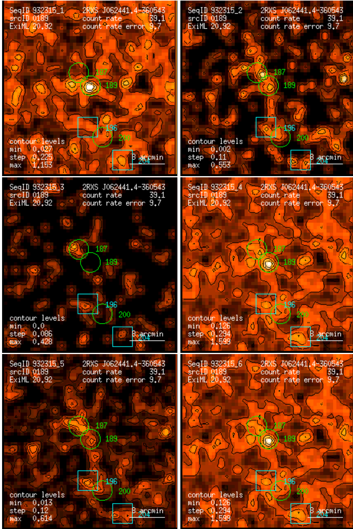
Figure 189: RASS 932315: detection 0189: band rate images, Gaussian filter: (1) PSPC channels 11 – 41, (2) 52 – 90, (3) 91 – 201, (4) 11 – 235, (5) 52 – 201, (6) 11 – 201. Broad band rates in counts/ks. Band rate contour levels in counts/ks/arcmin 2 .
