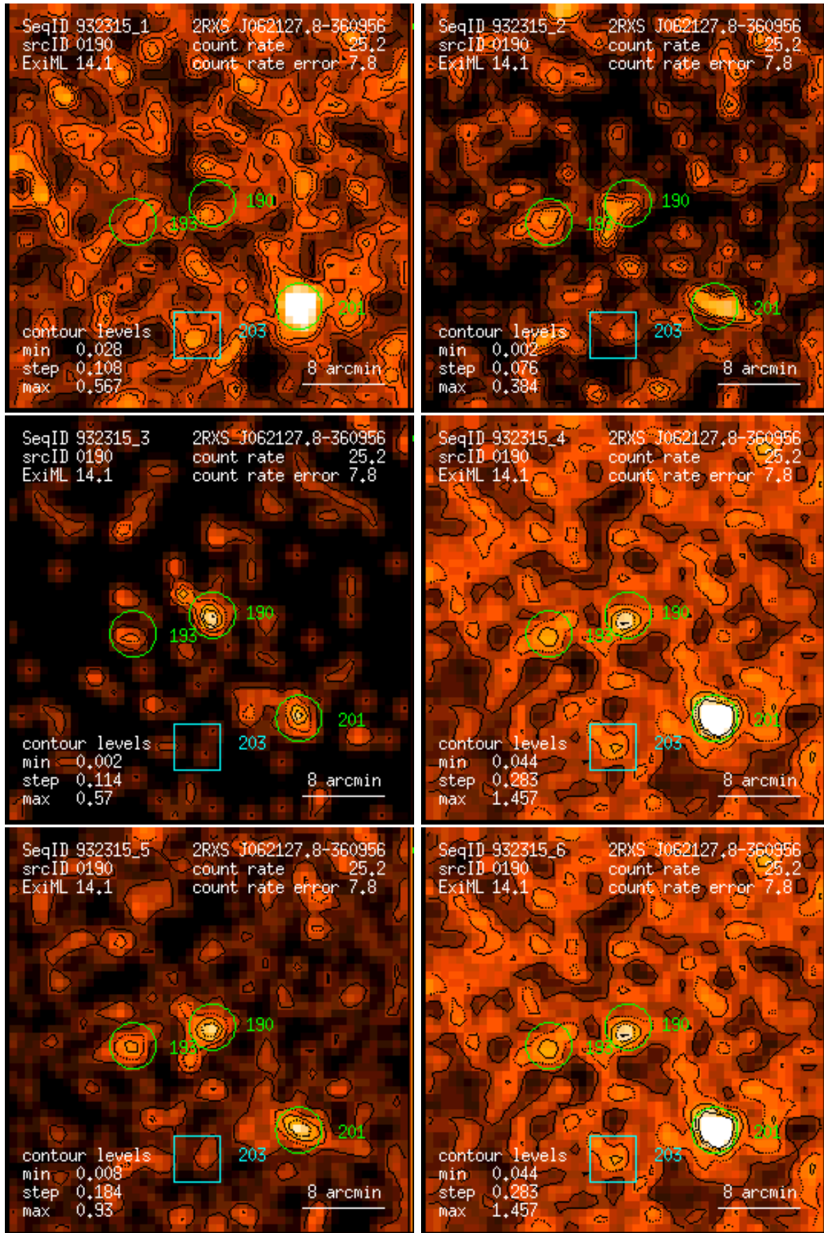
Figure 190: RASS 932315: detection 0190: band rate images, Gaussian filter: (1) PSPC channels 11 – 41, (2) 52 – 90, (3) 91 – 201, (4) 11 – 235, (5) 52 – 201, (6) 11 – 201. Broad band rates in counts/ks. Band rate contour levels in counts/ks/arcmin 2 .
