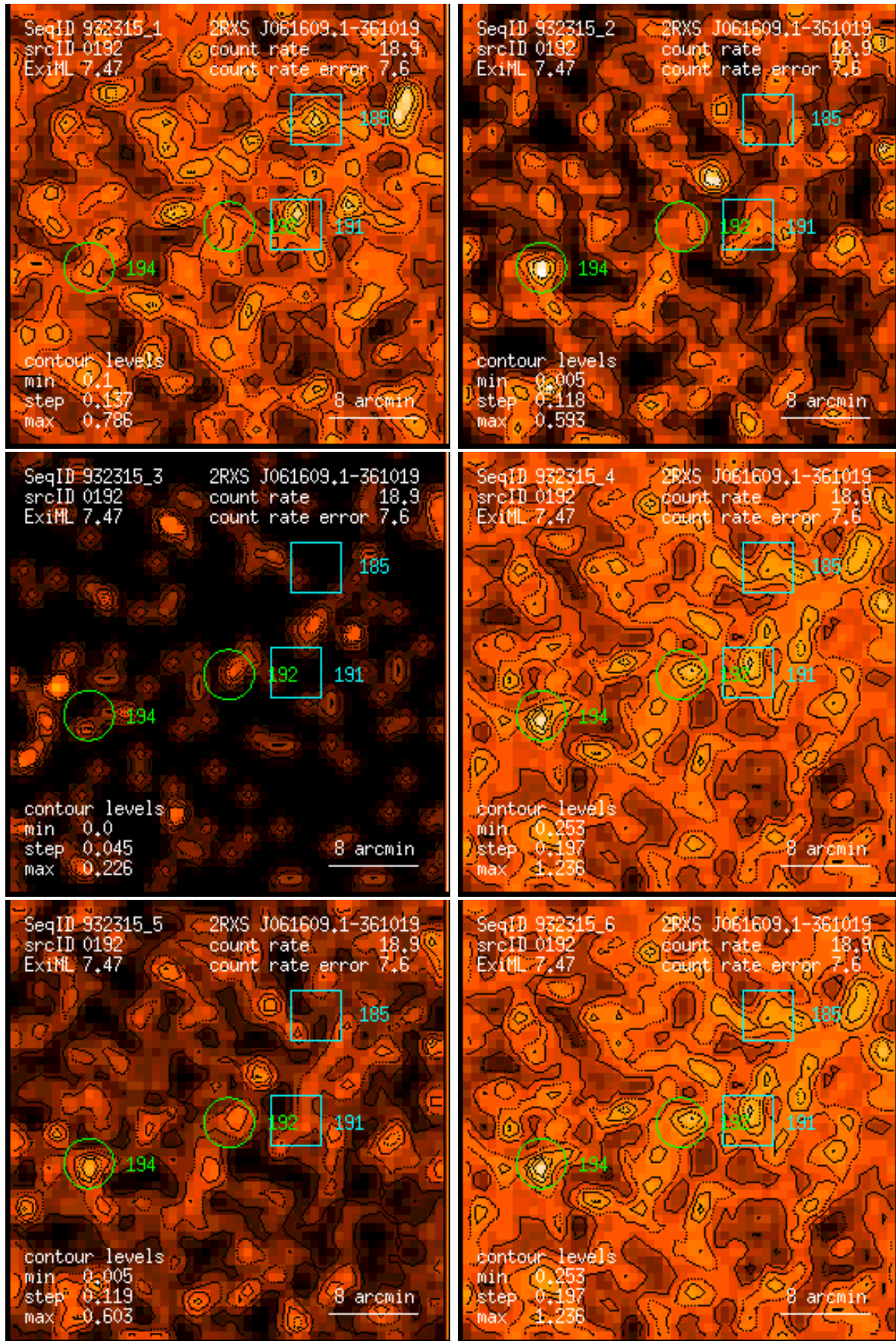
Figure 192: RASS 932315: detection 0192: band rate images, Gaussian filter: (1) PSPC channels 11 – 41, (2) 52 – 90, (3) 91 – 201, (4) 11 – 235, (5) 52 – 201, (6) 11 – 201. Broad band rates in counts/ks. Band rate contour levels in counts/ks/arcmin 2 .
