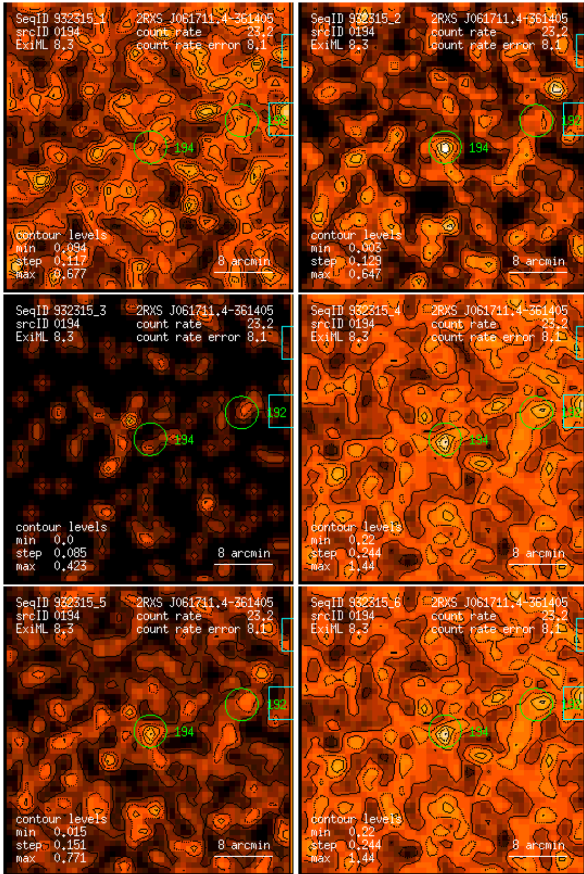
Figure 194: RASS 932315: detection 0194: band rate images, Gaussian filter: (1) PSPC channels 11 – 41, (2) 52 – 90, (3) 91 – 201, (4) 11 – 235, (5) 52 – 201, (6) 11 – 201. Broad band rates in counts/ks. Band rate contour levels in counts/ks/arcmin 2 .
