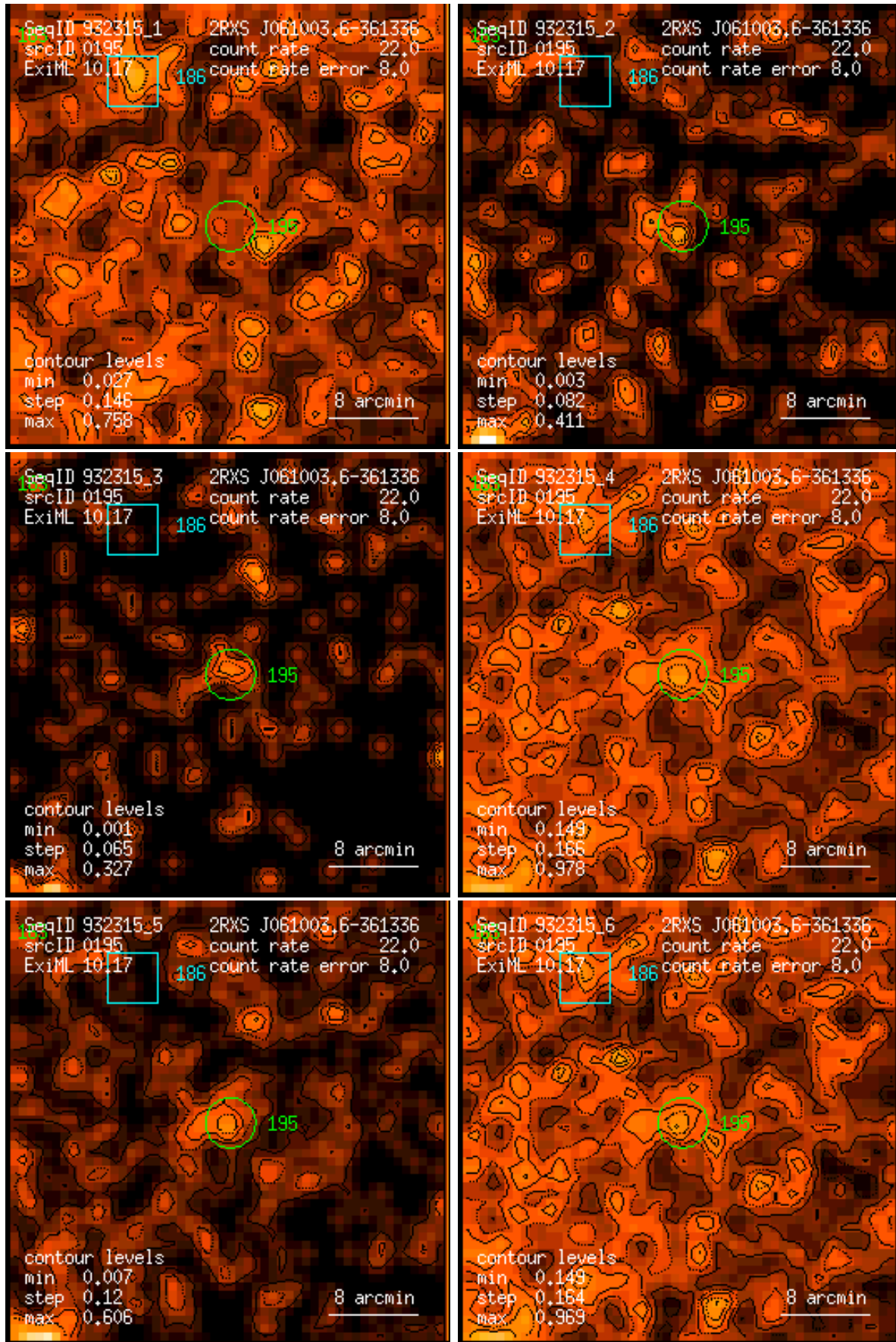
Figure 195: RASS 932315: detection 0195: band rate images, Gaussian filter: (1) PSPC channels 11 – 41, (2) 52 – 90, (3) 91 – 201, (4) 11 – 235, (5) 52 – 201, (6) 11 – 201. Broad band rates in counts/ks. Band rate contour levels in counts/ks/arcmin 2 .
