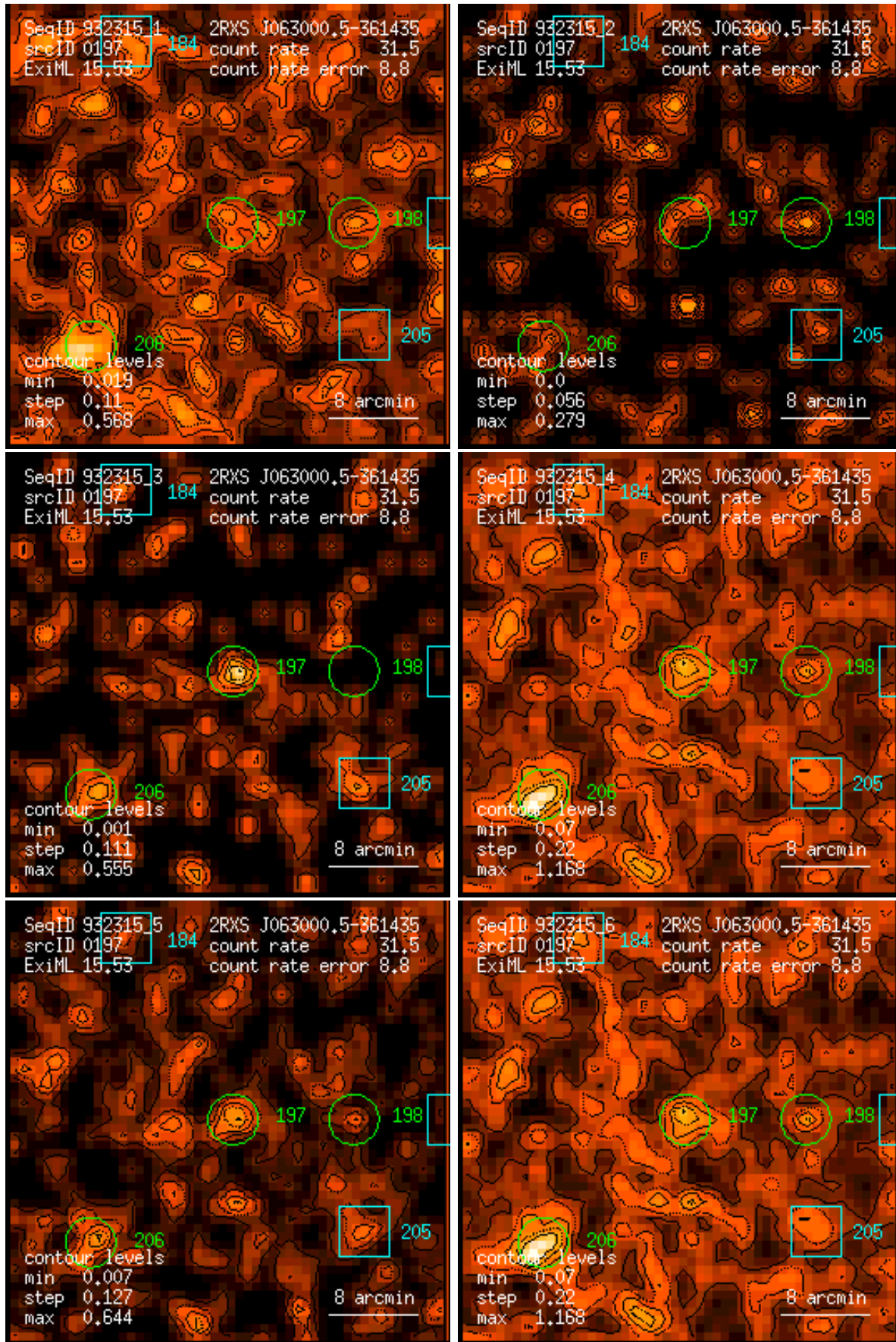
Figure 197: RASS 932315: detection 0197: band rate images, Gaussian filter: (1) PSPC channels 11 – 41, (2) 52 – 90, (3) 91 – 201, (4) 11 – 235, (5) 52 – 201, (6) 11 – 201. Broad band rates in counts/ks. Band rate contour levels in counts/ks/arcmin 2 .
