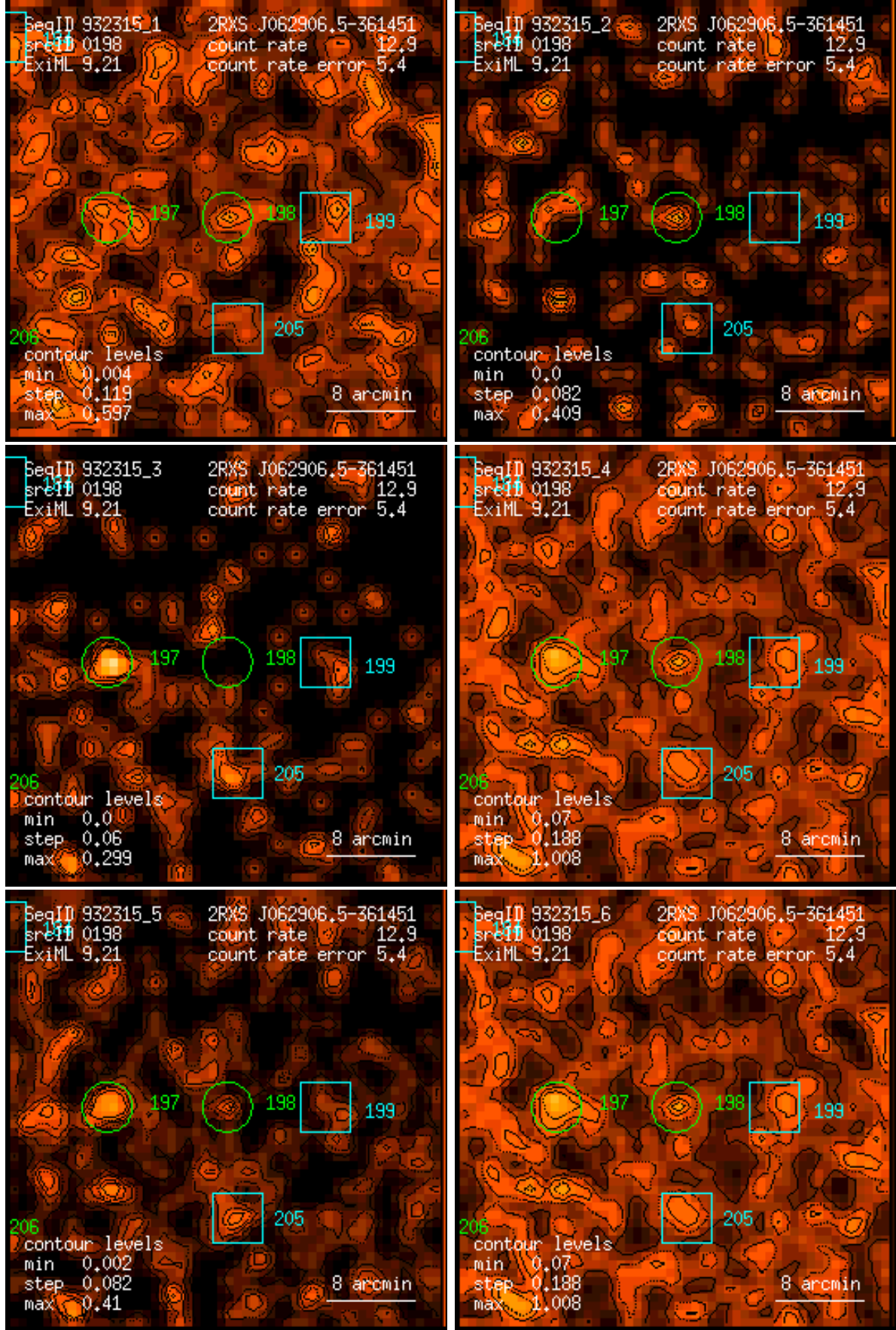
Figure 198: RASS 932315: detection 0198: band rate images, Gaussian filter: (1) PSPC channels 11 – 41, (2) 52 – 90, (3) 91 – 201, (4) 11 – 235, (5) 52 – 201, (6) 11 – 201. Broad band rates in counts/ks. Band rate contour levels in counts/ks/arcmin 2 .
